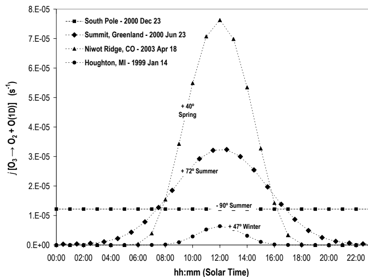
Fig. 1. Cloud-free J[O_3 + h\nu \rightarrow O_2 + O(^1D)] from TUV (Tropospheric Ultraviolet and Visible) radiation model for various latitudes and seasons at selected sites where snow photochemistry measurements have been made. Data shown for: South Pole (90° S, 23-December, 2000); Niwot Ridge, Colorado, USA (40° N, 18 April, 2003); Houghton, Michigan, USA (47° N, 14 January, 1999); and Summit, Greenland (74° N, 23 June, 2000).
