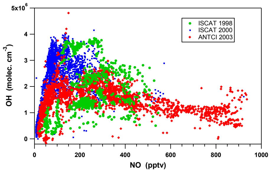
Fig. 9. OH versus NO at South Pole.
