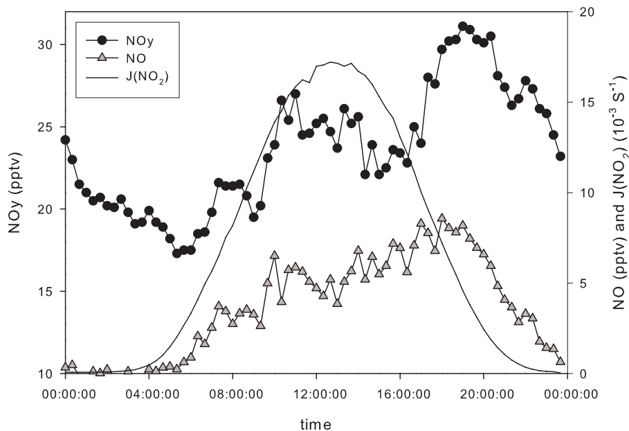
Fig. 7. Diurnal variation in NO y , NO and J-NO 2 measured at Neumayer Station, Antarctica, 1997, (Weller et al., 1999).
