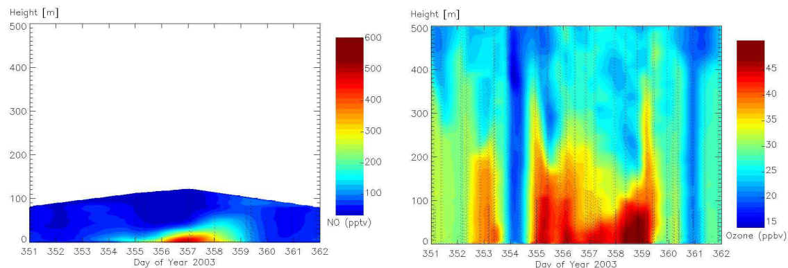
Fig. 11. Comparison of the vertical distribution of NO (left) and ozone (right) during Dec. 2003 at South Pole. These data are from concurrent vertical profile measurements of NO and ozone using a tethered balloon. (Figures adapted from Helmig et al., 2007a, 2007e).
