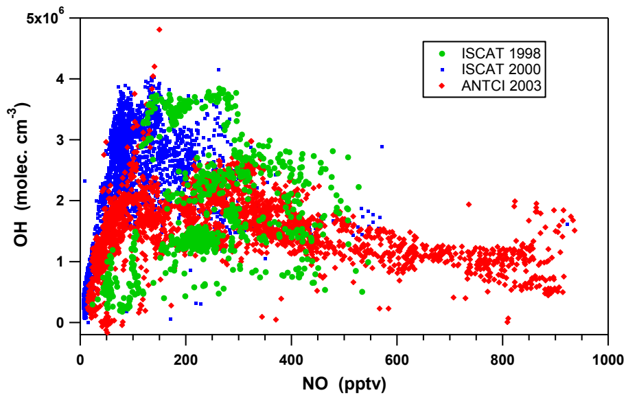
Fig. 9. OH versus NO at South Pole.
