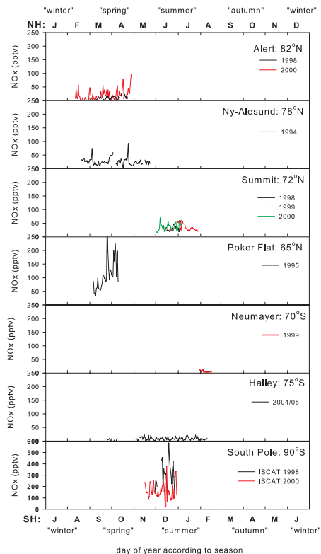
Fig. 6. As for Fig. 5, but for \text{NO}_x measurements – References as for Fig. 5. South Pole \text{NO}_x are based on calculated \text{NO}_2 values and measured \text{NO} values.
