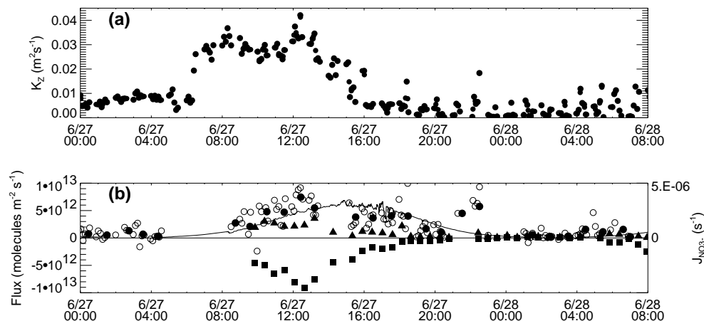
Fig. 4. (a) Eddy diffusivity measurements and (b) calculated fluxes (flux-gradient approach) during 27–28 June at Summit, Greenland. circles = \text{NO}_x , triangles = HONO, squares = \text{HNO}_3 , solid line = J(\text{NO}_3^-) . Positive values indicate an upward flux. (Reprinted from Honrath et al., Vertical fluxes of \text{NO}_x , HONO and \text{HNO}_3 above the snowpack at Summit, Greenland, Atmospheric Environment, 36, 2629–2640, 2002, with permission from Elsevier).
