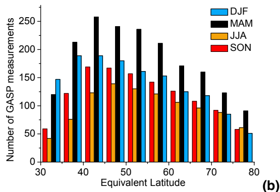
Fig. 9. (a) Climatological mean latitudinal distribution of lower stratospheric GASP ozone (5–50 K above the tropopause) (ppbv) as function of equivalent latitude and season. DJF (solid, blue), MAM (dashed, black), JJA (dashed-dot, orange), SON (dashed-dot-dot, red). Data are averaged over five degree bins. (b) Number of lower stratospheric GASP measurements at 5–50 K above the tropopause as function of equivalent latitude (five degree bins) and season. DJF (blue), MAM (black), JJA (orange), SON (red).
