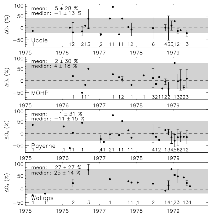
Fig. 12. Relative differences between quasi-monthly mean balloon and aircraft ozone in the UT ( \Delta\Theta < -2\text{K} ) for the period 1975–1979 (%). Comparison based on data from joint dates only. GASP ozone over Europe (Eastern USA) is evaluated against ozone at Uccle, MOHP, and Payerne (Wallops Island). Positive deviation indicates higher balloon than GASP ozone mixing ratio. Mean and median quasi-monthly mean differences are given in the upper left corners together with standard deviation and median absolute deviation, respectively. The range of the inner 90% is represented by the grey shading. Vertical bars denote standard deviation within a month if there is more than one concurrent date. At the bottom, the number of joint dates per month, from which quasi-monthly means and monthly standard deviations are calculated, is given for the period 1976–1979.
