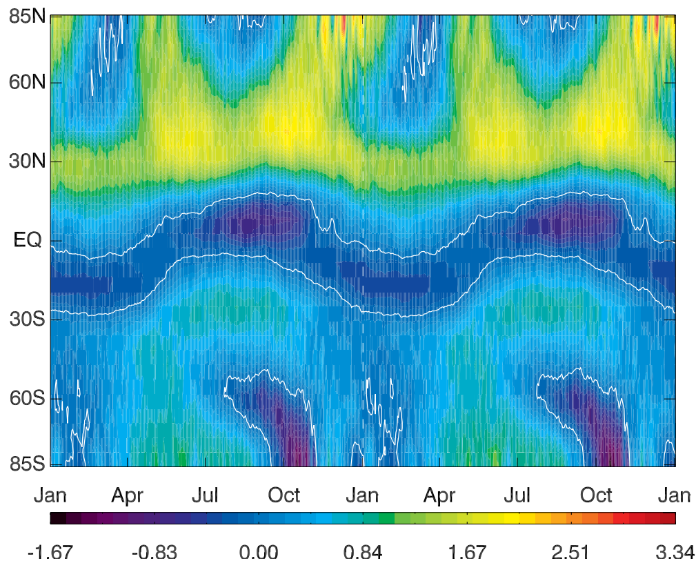
Fig. 11. Changes in the daily zonal mean total ozone column [Dobson Units] due to the mixed fleet aircraft emissions including aerosol emissions (AERO minus noAC), ranging from -1.67 DU to 3.34 DU.
