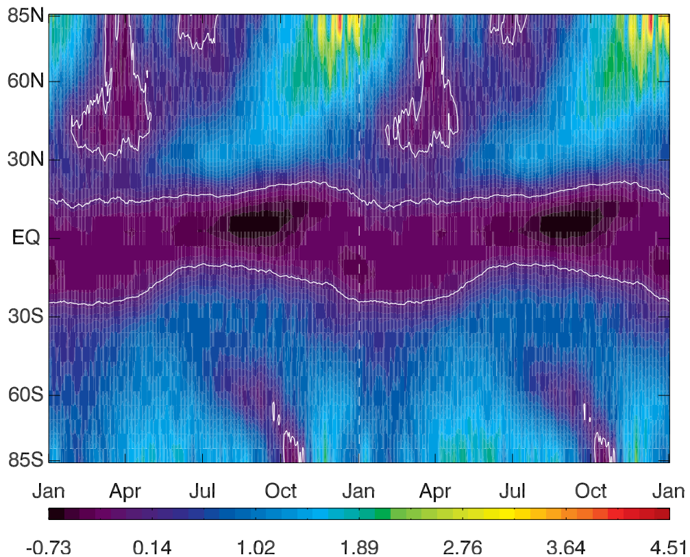
Fig. 12. Changes in the daily zonal mean total ozone column [Dobson Units] due to the mixed fleet aerosol emissions (AERO minus MIX).
