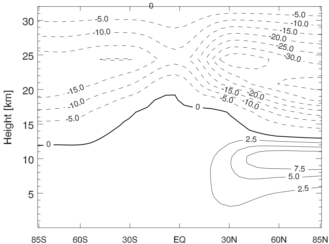
Fig. 3. Effect of aircraft emissions on \text{H}_2\text{O} , annual zonal mean (MIX minus noAC). Max: 629.69 ppbv.
