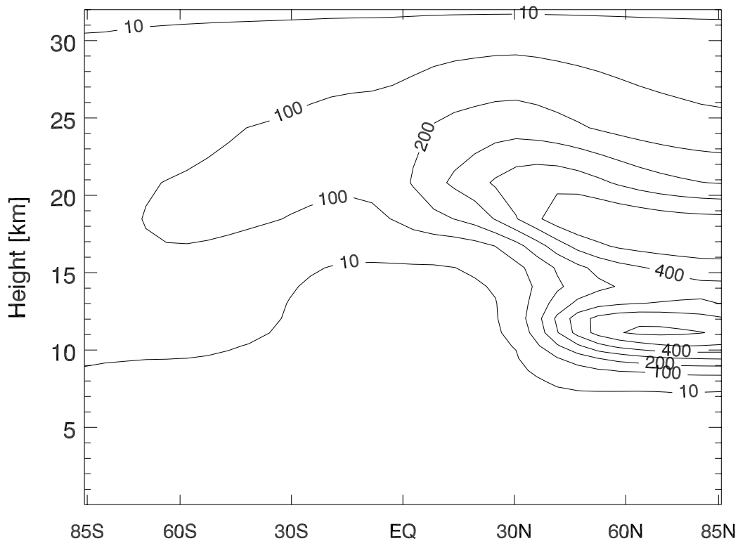
Fig. 2. Latitude and magnitude variation of the monthly mean maximum effect of aircraft emissions on \text{NO}_y (MIX minus noAC): 1.1 to 1.9 ppbv.
