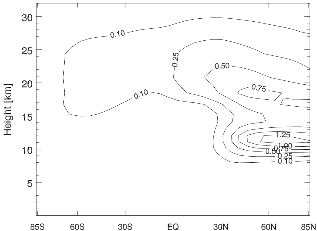
Fig. 1. Effect of mixed fleet aircraft emissions on \text{NO}_y , annual zonal mean (MIX minus noAC). Max: 1.35 ppbv.
