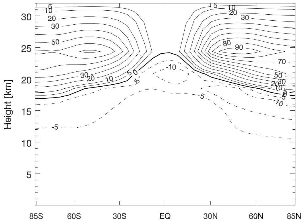
Fig. 13. Annual zonal mean effect of aircraft aerosol emissions on O 3 (AERO minus MIX).
