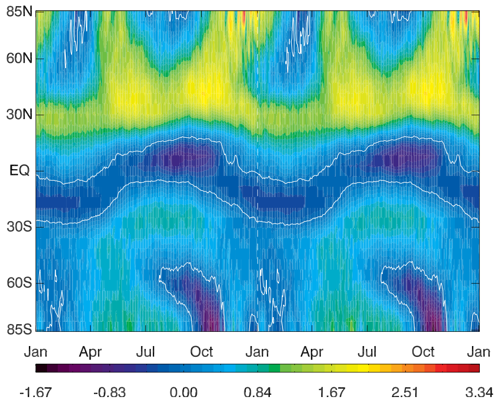
Fig. 10. Annual zonal mean effect of a mixed fleet with aerosol emissions on O_3 (AERO minus noAC).
