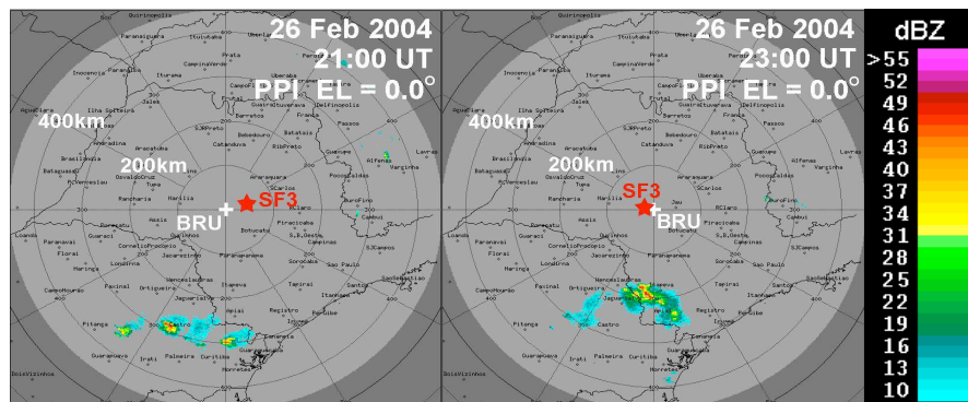
Fig. 11. SF3-flight. Thunderstorms over Paraná approaching from the south, as seen by the Bauru radar at 21:00 and 23:00 UT, respectively; surveillance PPI (450 km range) at 0° elevation. The star represents the SF3 balloon location at the time of the radar image, viz. 1 h after launch (left) and during its south-eastwards float (right), respectively.
