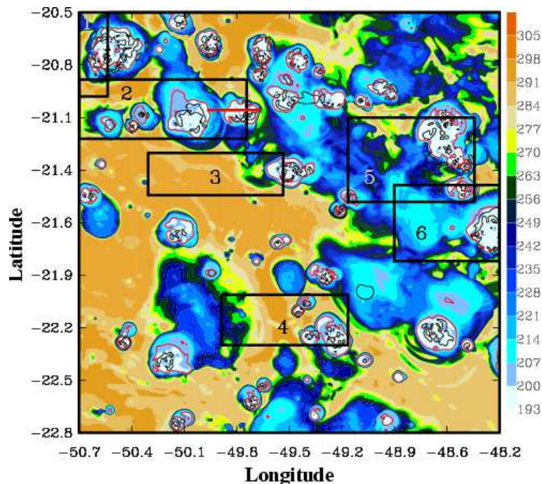
Fig. 4. High-resolution simulated fields in the model 4 domain at 18:30 UTC: BT at 10.8\ \mu\text{m} (color, K), BTD between 6.2\text{-} and 10.8\ \mu\text{m} band (3-K isoline in red), and water vapour mixing ratio over a 390-K potential temperature surface (4-ppmv isoline in black). The boxes indicate different sub-domains with occurrence of overshoots. The red line gives the position of the vertical cross-sections in Fig. 6.
