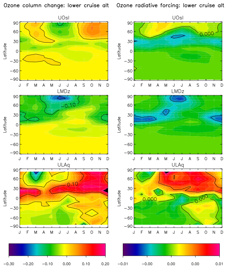
Fig. 4. Zonally averaged changes in (left) ozone column (DU) and (right) radiative forcing ( \text{Wm}^{-2} ) due ozone resulting from aircraft as a function of latitude and season in the case of lower cruise altitude.
