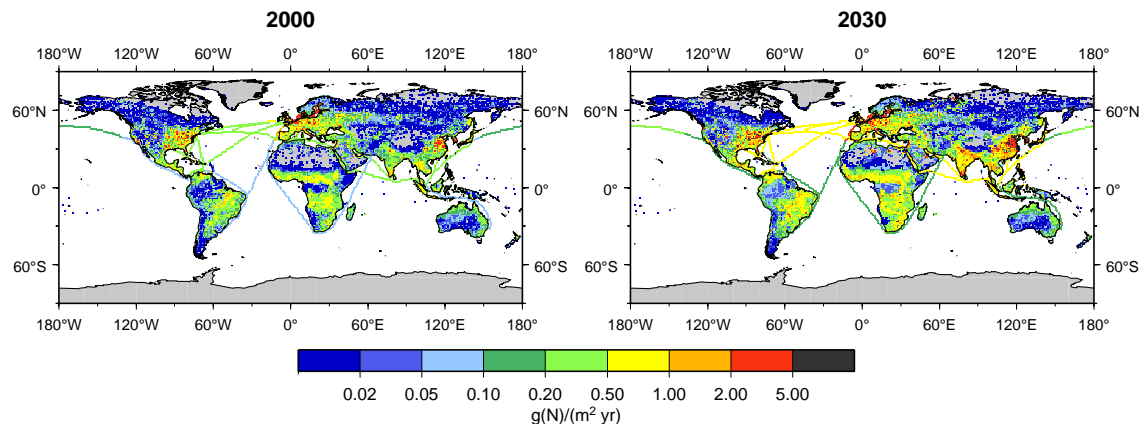
Fig. 1. Annual surface \text{NO}_x emissions including industry and power generation, traffic, domestic heating, and biomass burning (average 1997–2002 (van der Werf et al. (2004)) in \text{g(N)}/(\text{m}^2 \text{ yr}) . The left plot shows the emissions used as input for the model experiment S1 (year 2000, 38.0 \text{ Tg(N)}/\text{yr} total), the right plot the emissions for experiment S4s (year 2030, 67.6 \text{ Tg(N)}/\text{yr} total).
