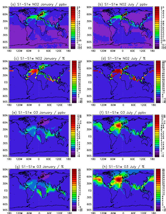
Fig. 3. Modelled ensemble mean near-surface \text{NO}_2 and ozone change between case S1 (year 2000) and S1w (year 2000 without ship emissions) in January (left) and July (right). 1st row shows absolute changes in near-surface \text{NO}_2 (a, b), 2nd row shows relative changes in near-surface \text{NO}_2 (c, d), 3rd row shows absolute changes in near-surface \text{O}_3 (e, f), and 4th row shows relative changes in near-surface \text{O}_3 (g, h).
