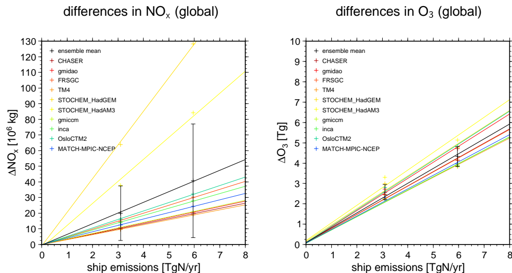
Fig. 7. Global total change in annual mean tropospheric \text{NO}_x burden (left) and ozone burden (right) due to ship emissions (S4–S4w and S4s–S4w) in each individual model (coloured lines) and the ensemble mean (black line). Inter-model standard deviations are shown as bars.
