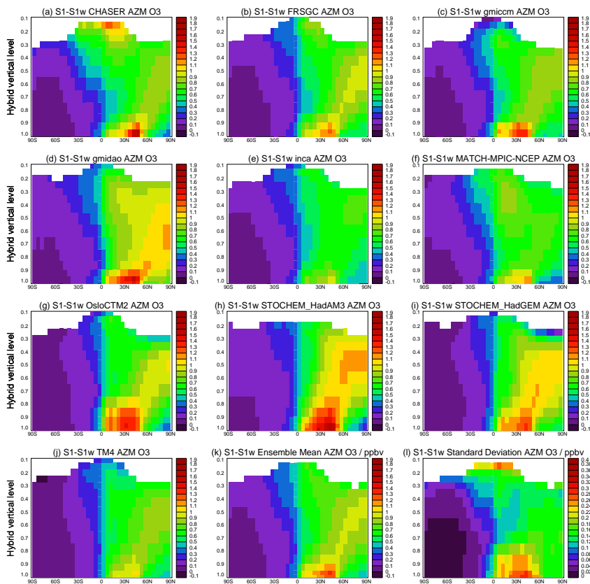
Fig. 2. Modelled zonal annual mean ozone change (ppbv) between case S1 (year 2000) and S1w (year 2000 without ship emissions): (a)–(i) individual models (k) ensemble mean (all 10 models) and (l) absolute standard deviations. Individual model results were interpolated to a common grid ( 5^\circ \times 5^\circ \times 19 levels) and masked at the chemical tropopause ( O_3 = 150 ppbv).
