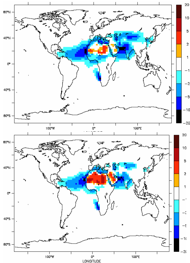
Fig. 9. TOA radiative forcing ( \text{Wm}^{-2} ) from mineral dust (SW+LW), the hematite is internally mixed and the top and bottom panels are for respectively 0.9 and 2.7% hematite (volume content).
