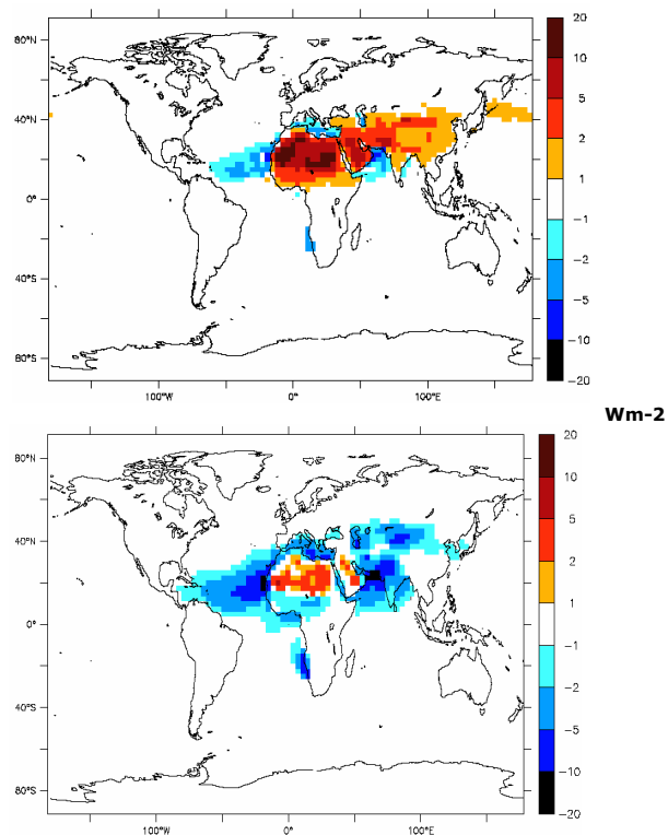
Fig. 7. Comparison of TOA radiative forcing of dust for 2 different hypotheses for dust refractive index: Top panel: Patterson and Volz; Bottom Panel: 1.5% by volume hematite content internally mixed.
