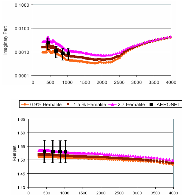
Fig. 4. Real and imaginary parts of mineral aerosol refractive indices. The solid triangles and squares are for an internal mixture with respectively 0.9%, 1.5 and 2.7% hematite by volume. The hematite is present as a coating over the other 5 other minerals (calcite, quartz, illite, kaolinite and montmorillonite). The refractive index of the internal mixture is computed using the Maxwell Garnett approximation given in Eq. (1) (see text). The AERONET measurements are the ones reported by Dubovik (2002). Uncertainties are 0.04 on the real part of the refractive index and 50% on the imaginary part (Dubovik, 2002, and personal communication).
