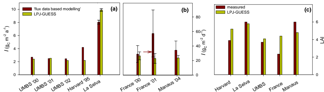
Fig. 4. (a) and (b): Annual (a) and daily (b) simulated canopy isoprene emissions ( I ) and estimates derived from flux measurements (“flux-data based modelling”) from five different forest sites (UMBS, Harvard, La Selva, France, Manaus). Numbers indicate the year of measurements and simulation. At La Selva the data are average and standard deviation for the period 1998–2000. For the French and Manaus sites, data and model output are average daily emission obtained from ca. 2-week long campaigns. These were performed during June/July 2001 and 2002 in France, and September 2004 at the Manaus tower. An arrow indicates average daily isoprene emissions for the first half of the 2001 measurement campaign in France. A description of the sites and data sets is provided in the text.
