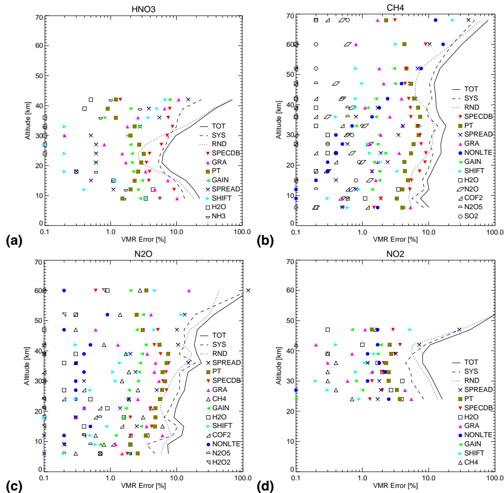
Fig. 8. As Fig. 7, showing retrieval error budgets for nitric acid, methane, nitrous oxide and nitrogen dioxide.
