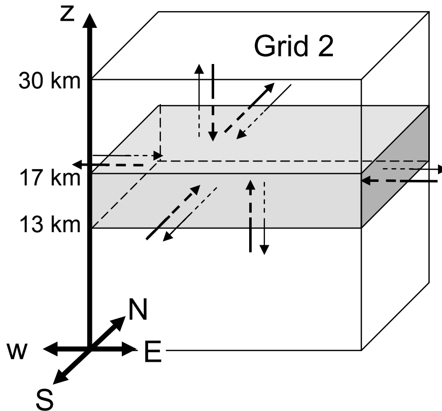
Fig. 7. Schematic of the box used to calculate the ozone budget in the TTL (shaded domain delimited at the bottom by the 13 km level, at the top by the 17 km level and on the sides by the boundary of Grid 2). The net contribution (inflowing flux or outflowing flux) on the budget for each side of the domain is indicated by the sense of the corresponding bold arrows.
