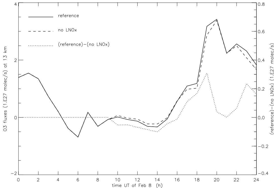
Fig. 9. O_3 instantaneous fluxes at the bottom of the domain shown in Fig. 7 between 8 February, 00:00 UT and 9 February, 00:00 UT for the “reference” (solid line) and the “no LNO_x ” (dashed line) runs (left y-axis scale). The difference between these two fluxes is also shown (right y-axis scale).
