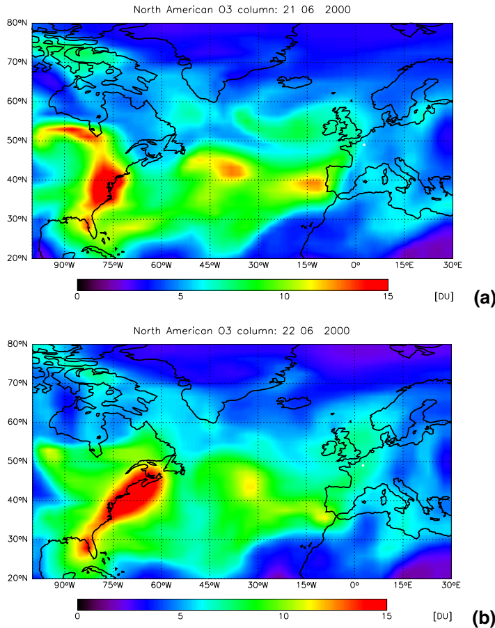
Fig. 11. LRT2 : (a) and (b) Daily averaged North American ozone column on 21 and 22 June. (c) O 3 mean and standard deviation for the period 21–23 June at Paris from GEOS-CHEM (solid line) and MOZAIC (dashed line). (d) GEOS-CHEM profiles at Paris on 21–23 June, North American O 3 (dash-dotted line) and stratospheric O 3 (dashed line). (e) MOZAIC profiles at Paris on 21–23 June.
