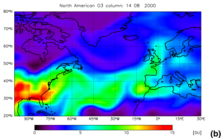
Fig. 13. LRT9 : North American ozone column on (a) 13 August and (b) 14 August 2000. (c) O 3 mean and standard deviation for the period 13–15 August at Paris from GEOS-CHEM (solid line) and MOZAIC (dashed line). (d) GEOS-CHEM profiles at Paris on 13–15 August, North American O 3 (dash-dotted line) and stratospheric O 3 (dashed line). (e) MOZAIC profiles at Paris on 13–15 August.
