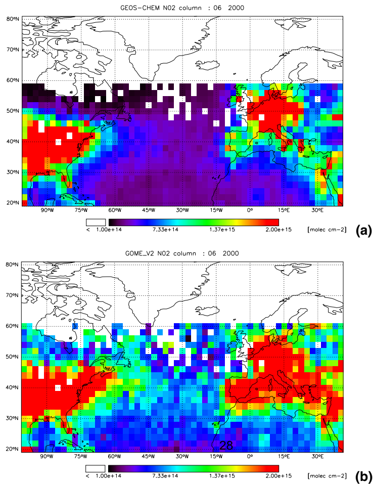
Fig. 2. Mean cloud-filtered tropospheric NO 2 columns in June 2000 from: (a) GEOS-CHEM and (b) GOME. (c) scatter plot GEOS-CHEM vs. GOME.
