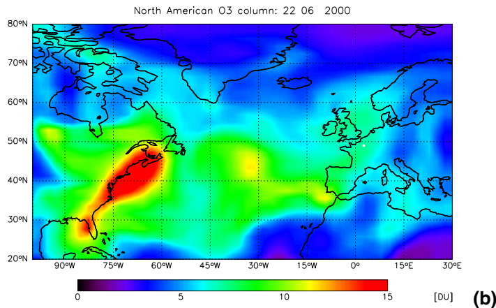
Fig. 11. LRT2 : (a) and (b) Daily averaged North American ozone column on 21 and 22 June. (c) O 3 mean and standard deviation for the period 21–23 June at Paris from GEOS-CHEM (solid line) and MOZAIC (dashed line). (d) GEOS-CHEM profiles at Paris on 21–23 June, North American O 3 (dash-dotted line) and stratospheric O 3 (dashed line). (e) MOZAIC profiles at Paris on 21–23 June.
