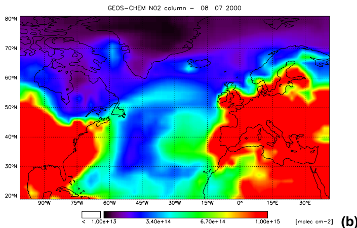
Fig. 7. Illustration of LRT4 event: (a) GEOS-CHEM CO at 700 hPa on 8 July, (b) GEOS-CHEM NO 2 column on 8 July, (c) GEOS-CHEM mean sea level pressure and 500 hPa winds on 8 July.
