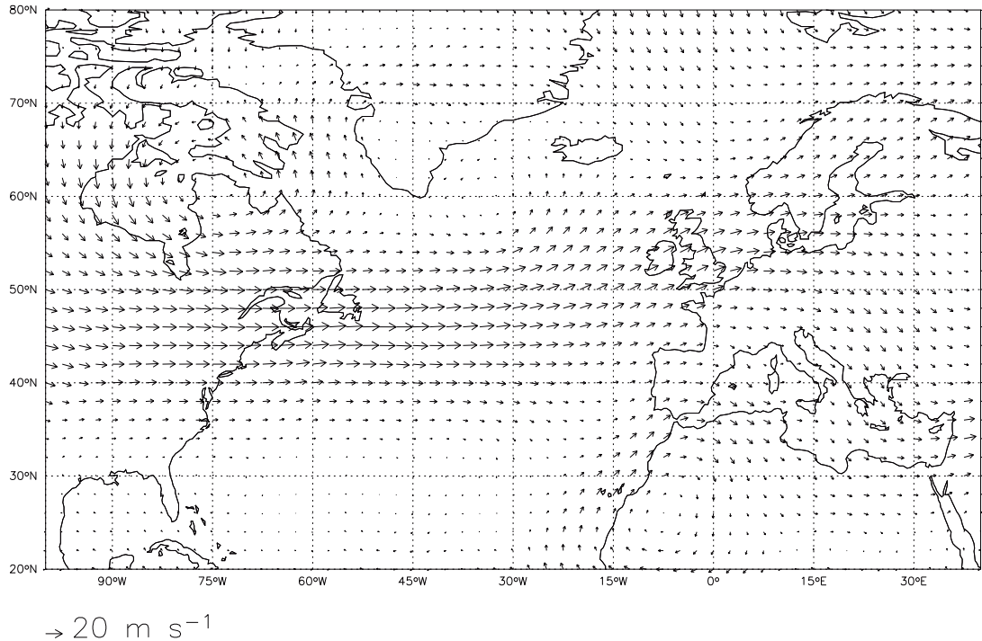
Fig. 4. GEOS-CHEM monthly mean winds at 500 hPa for: (a) June 2000, (b) July 2000, and (c) August 2000.
