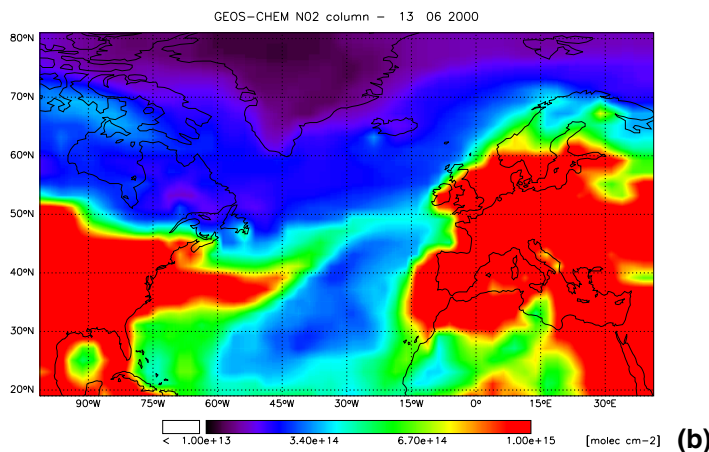
Fig. 5. Illustration of LRT1 event: (a) GEOS-CHEM CO column on 13 June, (b) GEOS-CHEM NO 2 column on 13 June, (c) MOPITT CO column for 9–13 June, (d) GOME NO 2 column on 11–13 June and (e) GEOS-CHEM mean sea level pressure and 500 hPa winds on 13 June.
