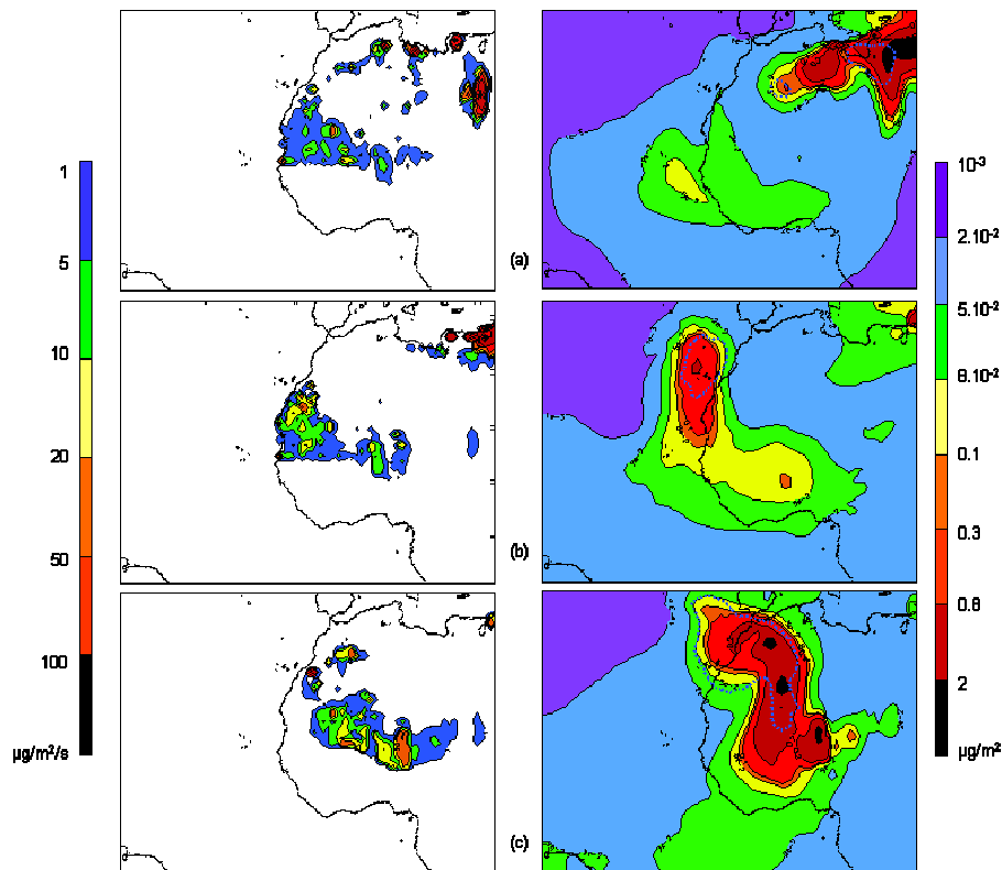
Fig. 3. Averaged mass fluxes ( \mu\text{g}/\text{m}^2/\text{s} ) and integrated dust loading ( \mu\text{g}/\text{m}^2 ) for the dust event from 4 to 11 January 1993 (a), from 6 to 10 January 1993 (b) and from 16 to 25 January 1993 (c). The dotted line on the right-hand figures represents the limits of dust concentrations with calcite content >2.10^{-2} \mu\text{g}/\text{m}^3 at the surface.
