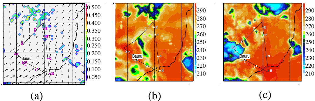
Fig. 3. (a) Simulated convective tendency for NO in pptv/s at 12 km, (b) 10.7 μm BTs (K) obtained from the Meso-NH simulation and (c) 10.7 μm BTs (K) obtained from GOES-12 observation on 3 March 2004 at 12:00 UTC. Black line displays the track of flight 9.
