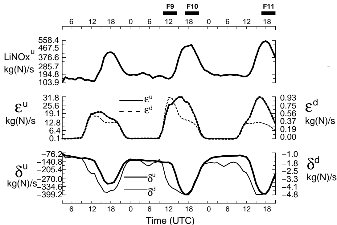
Fig. 11. Time evolution of simulated convective fluxes from 03:00 UTC 2 March till 21:00 UTC 4 March summed over the domain shown in Fig. 3, for the layer from 4 to 16 km height, in kg(N)/s.
