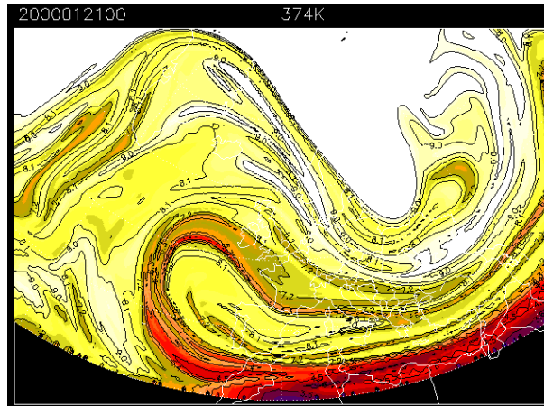
Fig. 4. PV map on a geographical sector including Europe. The potential vorticity is given for potential temperature corresponding to the top (374 K) and the bottom (367 K) part of the cloud.
