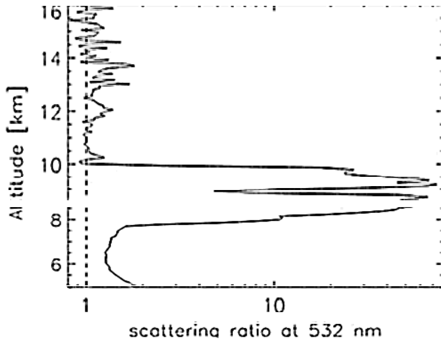
Fig. 2. Mean vertical backscattering ratio profile obtained with the lidar at OHP from 20:50 to 22:00 UT on 20 January 2000.
