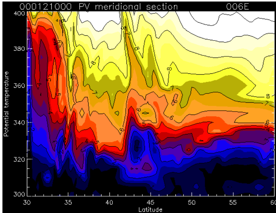
Fig. 3. PV meridional section, for latitudes from 30 to 60° N, at the OHP longitude, as deduced from the MIMOSA model for 20 January at midnight. The vertical structure is given for potential temperature from 300 to 400 K. The light-blue-purple colors correspond to air associated to the tropopause region, while orange yellow white colors indicate large PV values associated to stratospheric air.
