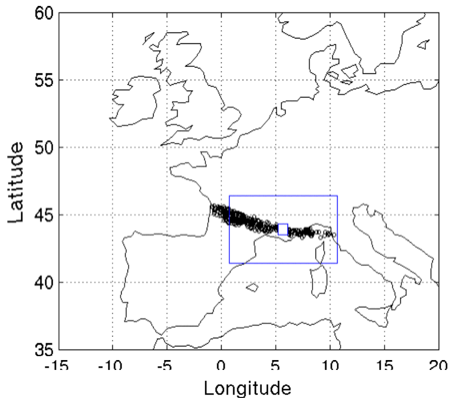
Fig. 5. Geographical position on 20 January 2000 at 18:00 of air parcels released at the altitude of the cirrus and that have gone below the thermal tropopause (backwards in time). The rectangle box corresponds to the spatial domain where back-trajectories were initialized.
