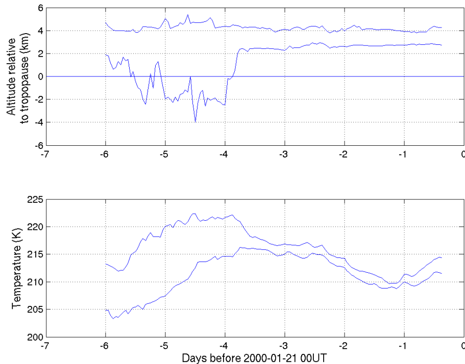
Fig. 6. Envelopes of altitude relative to the tropopause (top panel), and of the corresponding temperatures (bottom panel), for a cluster of air back-trajectories, starting from OHP on 20 January at night. Simulations are based on meteorological analyses and FLEXPART simulations.
