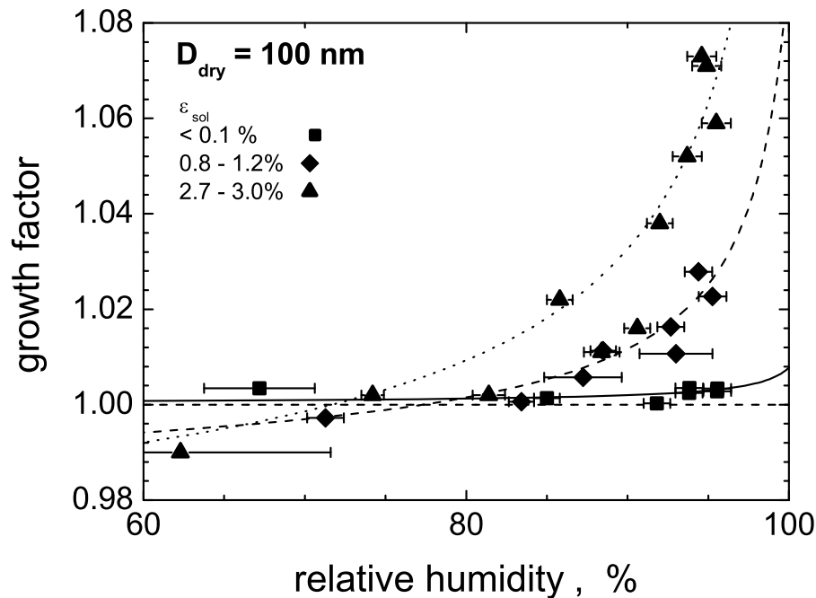
Fig. 10. Humidity growth of particles of initial size D_{dry}=100 nm as a function of relative humidity for low, medium and high fuel sulphur cases; lines represent growth curves determined from Köhler theory for the indicated volume fractions of soluble matter \epsilon_{sol} .
