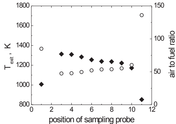
Fig. 1. Combustor exit temperature T_{exit} (filled symbols) and ratio of air to fuel (open symbols) for the sampling probe positions on the combustor exit nozzle plane (upper panel) during operation at old cruise conditions.
