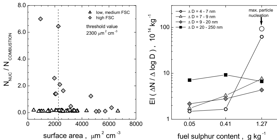
Fig. 9. Left: ratio of nucleated particles N_{NUC} of size D < 10 \text{ nm} to combustion particles N_{COMBUSTION} of size D \geq 20 \text{ nm} as a function of the surface area of the pre-existing combustion aerosol; the dashed line denotes the threshold value for particle nucleation of 2300 \mu\text{m}^2 \text{cm}^{-3} . Right: number of particles per kg of consumed fuel in denoted diameter bins as a function of the fuel sulphur content.
