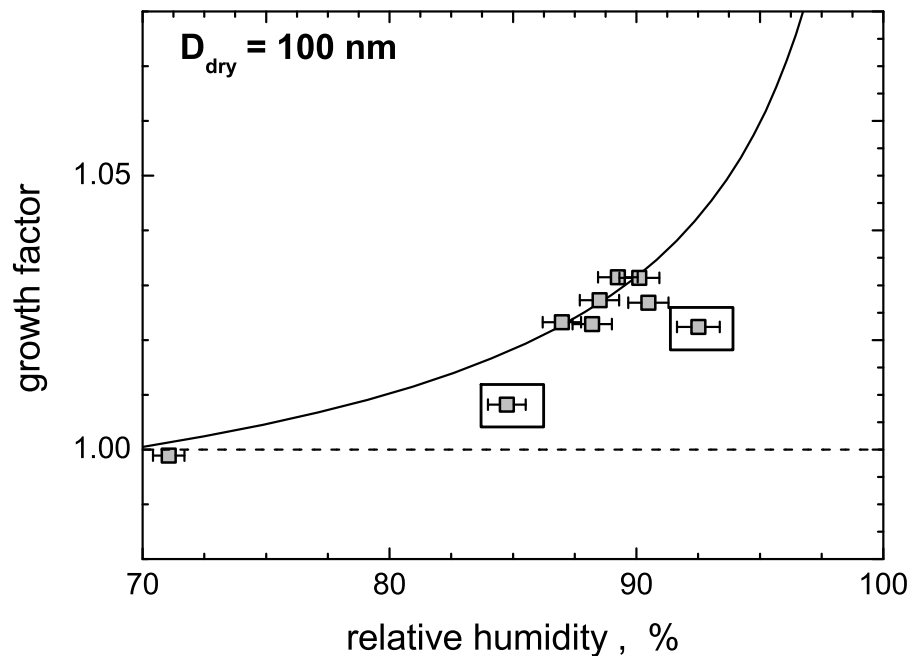
Fig. 13. Humidity growth of particles of initial size D_0=100 \text{ nm} as a function of relative humidity for the high fuel sulphur case; the indicated data points correspond to sampling points at the edge positions of the combustor exit nozzle plane.
