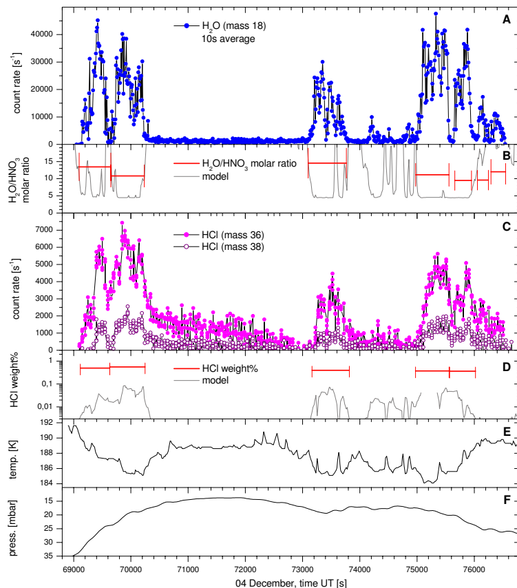
Fig. 2. (A) Water contained in PSC particles measured on mass 18 (H 2 O), averaged over 10 s. (B) H 2 O/HNO 3 molar ratios derived from measurements and model (Carslaw et al., 1995). (C) HCl contained in liquid PSC particles measured on masses 36 (H 35 Cl) and 38 (H 37 Cl). (D) HCl weight% derived from measurements and model (Carslaw et al., 1995). (E) Measured atmospheric temperature. (F) Measured atmospheric pressure.
