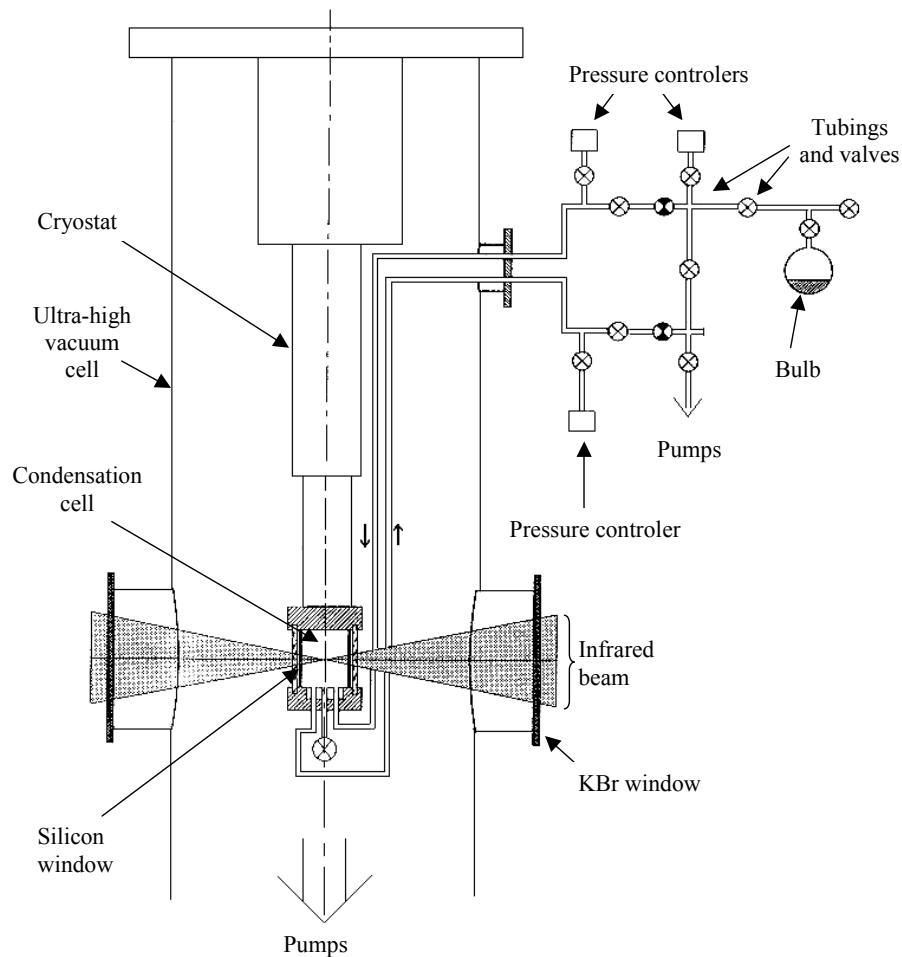
Fig. 1. Experimental set-up.
