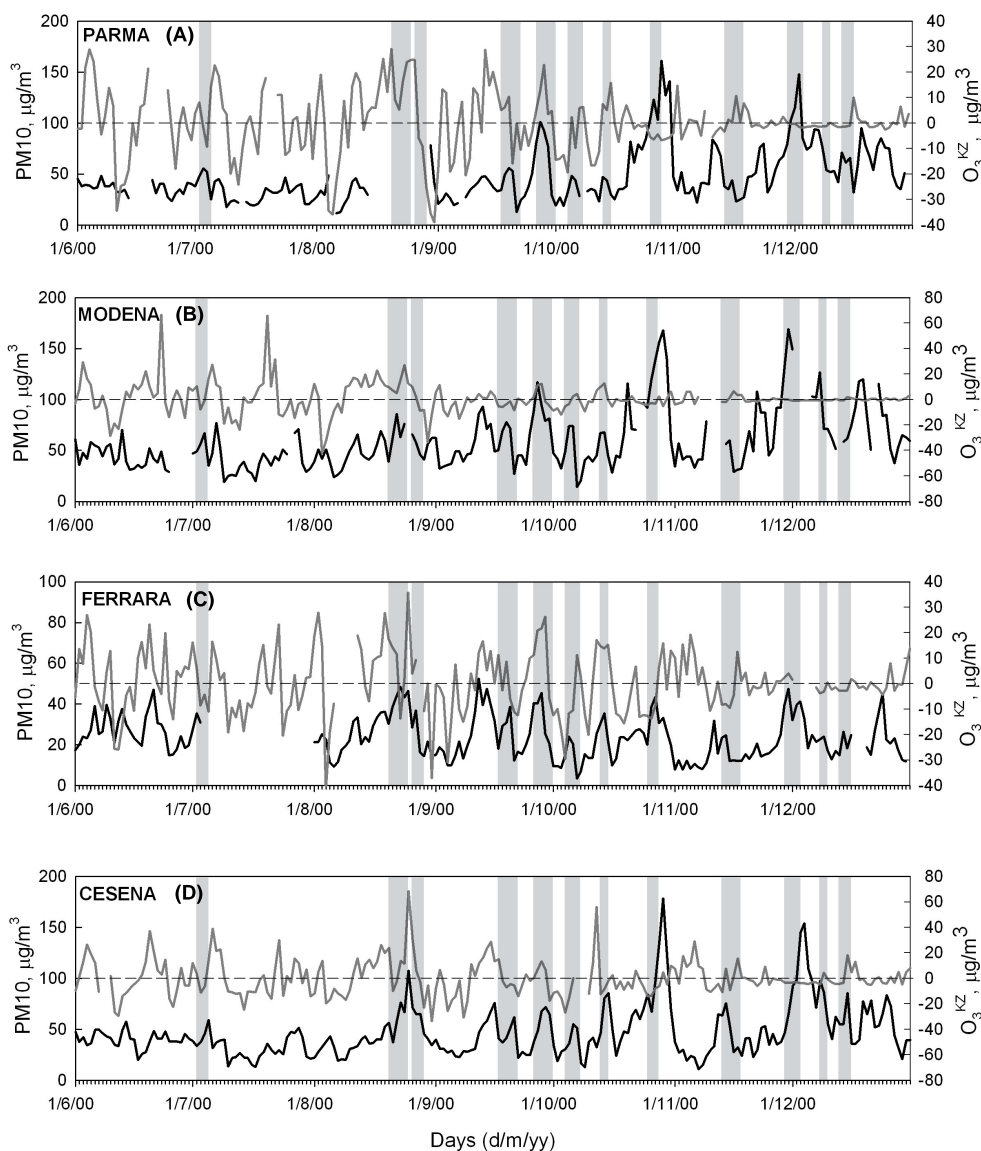
Fig. 8. Time series of PM 10 (black line) and O 3 KZ (grey line, see text for definition) concentration measured in the Po valley urban areas: Parma (A), Modena (B), Ferrara (C) and Cesena (D) from June to December 2000. Coloured bars represent the duration of the dust transport events as identified at the MTC station.
