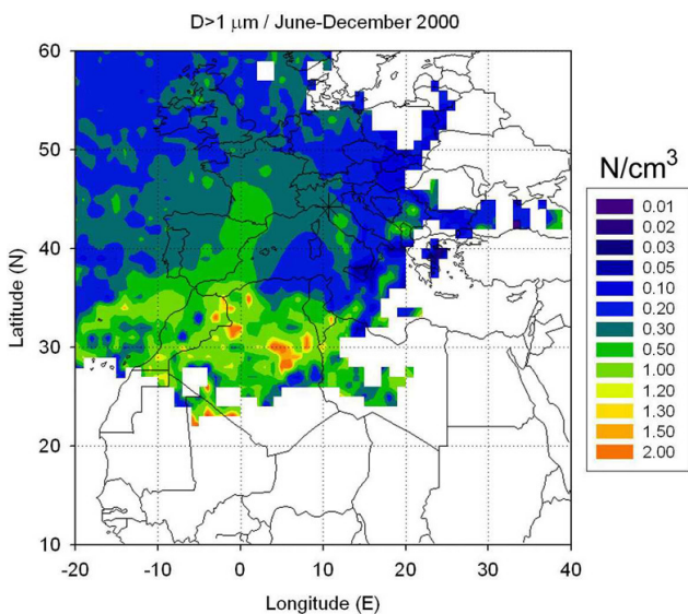
Fig. 6. Number concentration ( N/\text{cm}^3 ) field for coarse aerosol ( D_p > 1 \mu\text{m} ) as obtained by the trajectory statistical analysis, June–December 2000.
