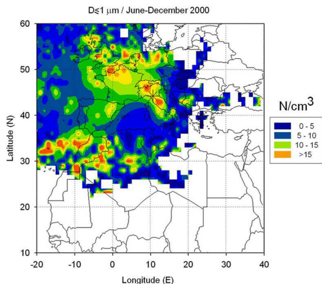
Fig. 5. Number concentration ( N/\text{cm}^3 ) field for fine aerosol ( D_p \leq 1 \mu\text{m} ) as obtained by the trajectory statistical analysis, June–December 2000.
