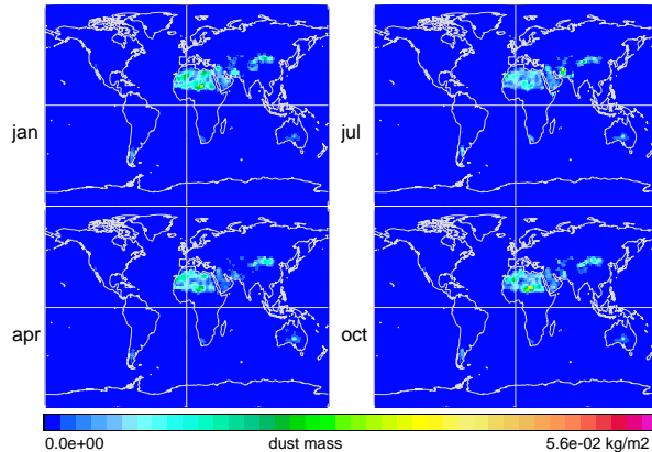
Fig. 1. Global fields of annual dust emission fluxes and dust emissions for four selected months (January, April, July and October). Dust emissions are given in \text{kg/m}^2 according to the linear color scale and its minimum and maximum values.
