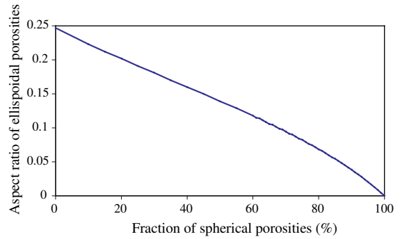
Fig. 14. Aspect ratio of ellipsoidal pores population versus fraction of spherical pores for a total porosity of 10% in the case of bi-modal microstructure.
