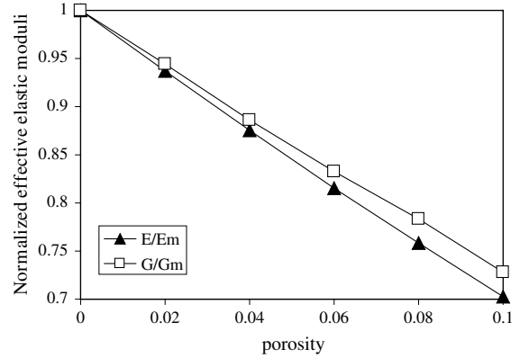
Fig. 4. Numerical results for ellipsoidal pores ( w = 0.2 ): normalized effective elastic moduli versus porosity.
