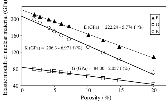
Fig. 12. Experimental data: elastic moduli of nuclear material versus porosity.
