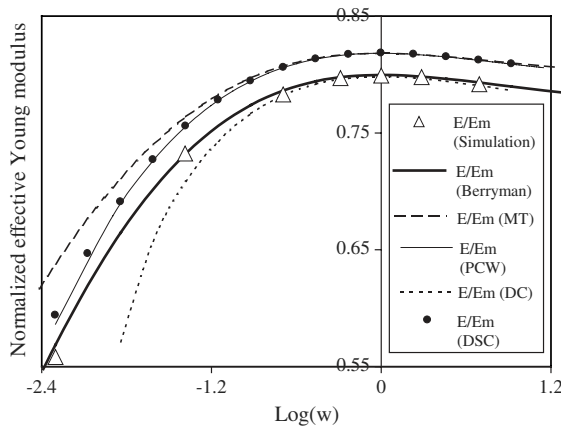
Fig. 8. Comparison between numerical results and various estimates (Berryman, Mori-Tanaka (MT), dilute case (DC), differential self-consistent (DSC), Ponte-Castañeda-Willis (PCW)) for spherical and ellipsoidal pores at f = 10\% : normalized effective Young modulus versus aspect ratio for density parameter lower than 1.
