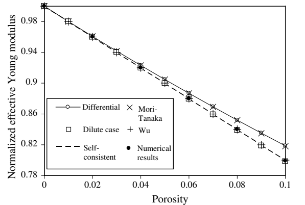
Fig. 6. Effective Young modulus versus porosity (spherical pores): comparison between various estimates and numerical results.
