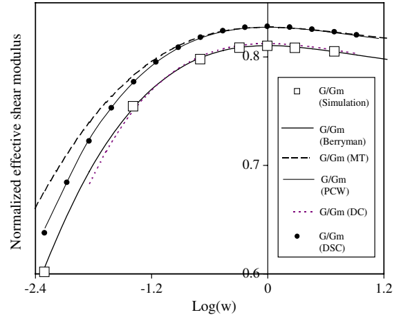
Fig. 9. Comparison between numerical results and various estimates (Berryman, Mori-Tanaka (MT), dilute case (DC), differential self-consistent (DSC), Ponte-Castañeda-Willis (PCW)) for spherical and ellipsoidal pores at f = 10\% : normalized effective shear modulus versus aspect ratio for density parameter lower than 1.
