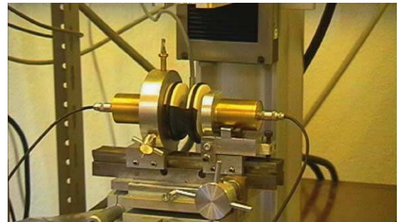
Fig. 11. Photography of the micro-echographic device.
