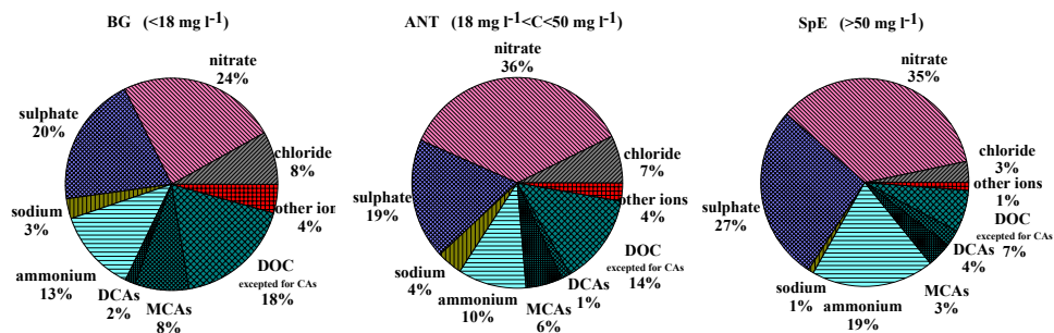
Fig. 4. Cloud water composition (in mg l -1 ) for ionic and organic compounds for the three different types of cloud event at PDD.
