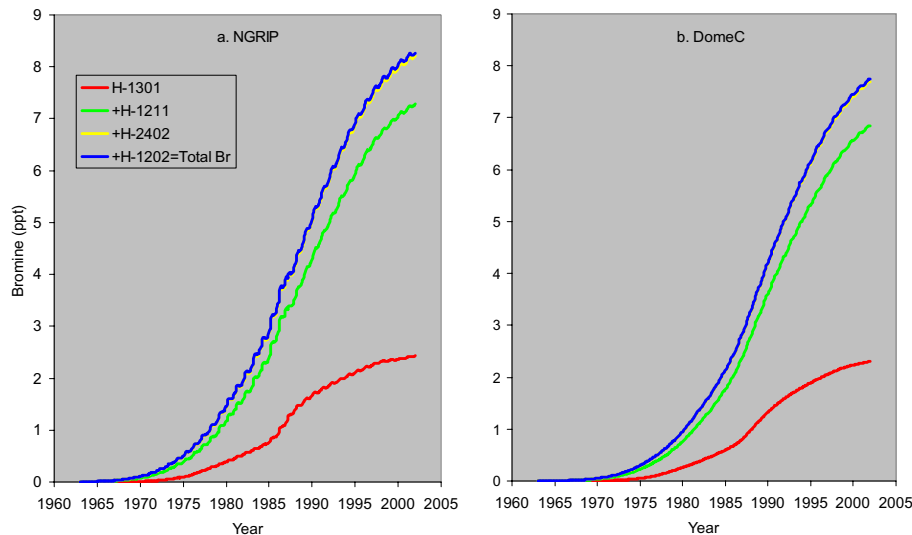
Fig. 6. Historical trends in atmospheric concentrations of organic bromine at (a) NGRIP, (b) Dome C. Red line is Br from H-1301 from Run A, green line is plus Br from H-1211 from run A+F, yellow line is plus Br from H-2402 from run A and blue line is plus Br from H-1202 from run A+F.
