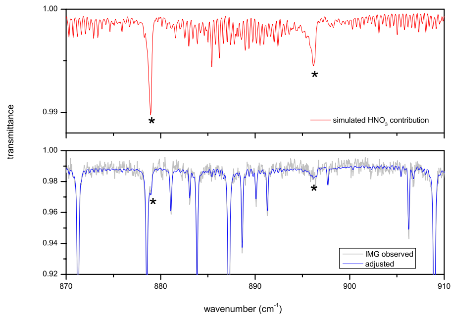
Fig. 5. Detection of HNO 3 from IMG data.
