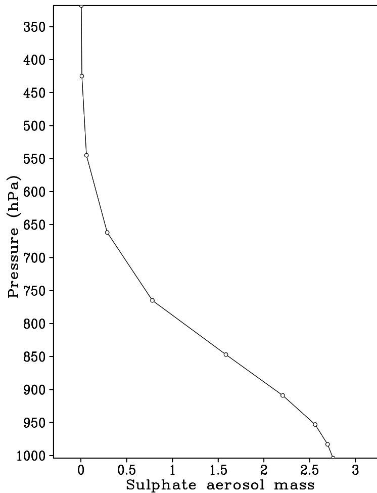
Fig. 9. Averaged vertical profile of sulphate aerosol mass ( \mu\text{g m}^{-3} ) over the entire INDOEX region for the IFP.
