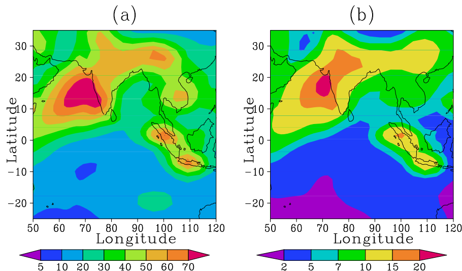
Fig. 10. Spatial distribution of particle number concentration (divided by 100) for January to March at surface in (a) Aitken mode and (b) accumulation mode concentration (particle \text{cm}^{-3} ).
