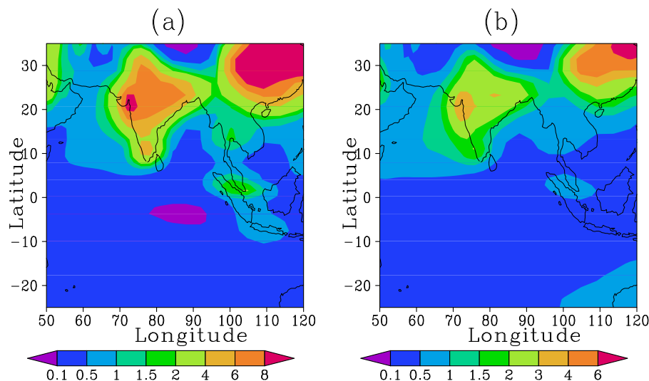
Fig. 7. Average \text{SO}_2 distribution for January to March 1999 for the INDOEX domain: (a) surface concentration ( \mu\text{g SO}_2 \text{ m}^{-3} ); (b) column burden ( \text{mg S m}^{-2} ).
