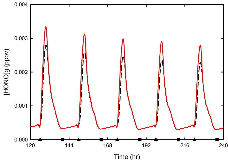
Fig. 1. Diurnal behaviour of gas phase HONO during the exposure of monodispersed droplets (with a radius of 0.1 \mu\text{m} and L = 50 \mu\text{g m}^{-3} ) containing initially 10^{-8} \text{M} aromatics. The multiphase chemistry was activated between 6:00 and 10:00 am. Solid line is with the charge exchange reactions between \text{NO}_2 and dissociated hydroxyl substituted aromatics. The dashed line is the base case without these reactions (left scale). Triangles and squares on the x -scale are indicating sunrise and sunset respectively.
