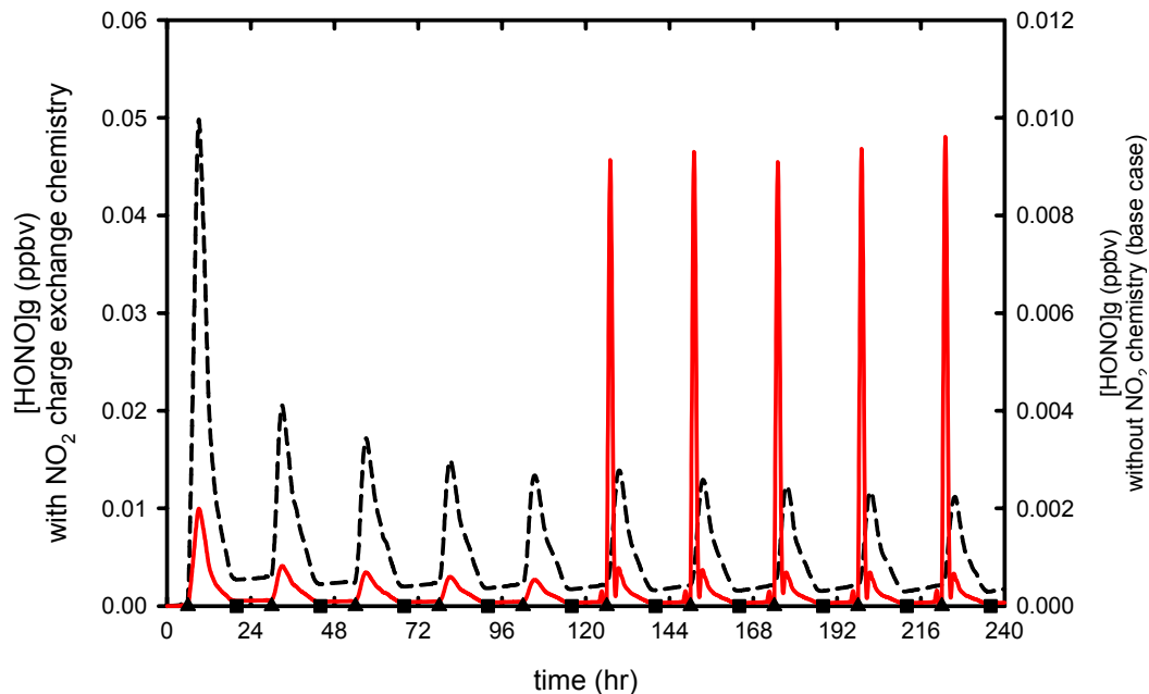
Fig. 2. Diurnal behaviour of gas phase HONO during the exposure of monodispersed droplets (with a radius of 0.1\ \mu\text{m} and L = 50\ \mu\text{g m}^{-3} ) containing initially 10^{-3}\ \text{M} aromatics. The multiphase chemistry was activated between 6:00 and 10:00 am and started on the 5th day. Solid line is with the charge exchange reactions between NO 2 and dissociated hydroxyl substituted aromatics (left scale). The dashed line is the base case without these reactions (right scale). Triangles and squares on the x-scale are indicating sunrise and sunset respectively.
