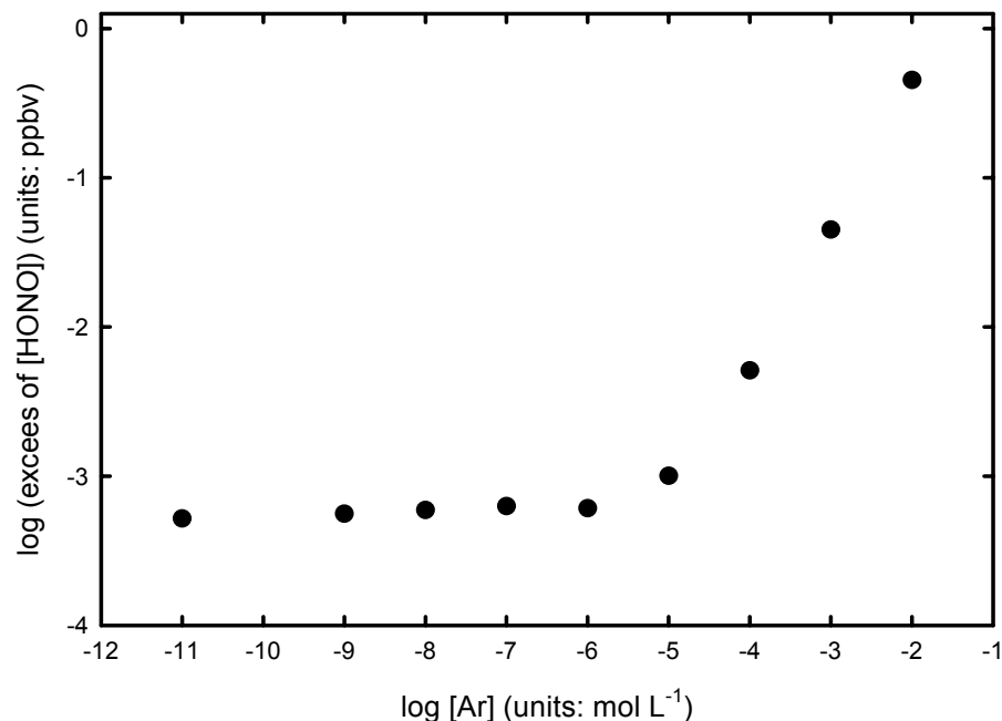
Fig. 3. Logarithm of the excess of gas phase HONO concentrations (expressed in nmol/mol) compared to the base case as a function of aromatic initial concentrations (in molar) determined at maximum HONO concentration. The excess of gas phase HONO is defined as the difference in concentration between the base case and simulations considering the charge exchange reactions between NO 2 and dissociated hydroxyl substituted aromatics.
