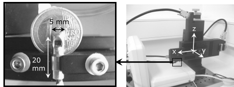
Figure 4. Micro camera compared with a coin of 1 euro (left), xyz stage (right).
