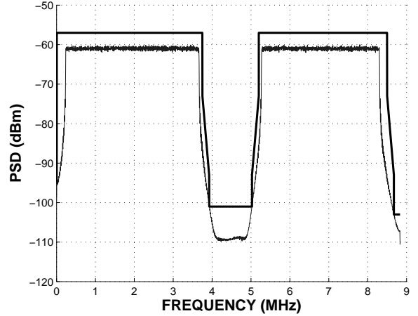
Fig. 4. Output PSD after the optimum distribution of number of taps amongst the tones
