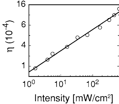
Fig. 4. Intensity dependence of the diffraction efficiency (on a square-root and logarithmic scale). The theoretical line is according to relation (5) with parameters \alpha=1730 \text{ cm}^{-1} (from Ref. 16), \Delta n=1.2 \times 10^{-4} , I_{\text{ref}}=0.2 \text{ mW/cm}^2 ( \lambda=488 \text{ nm} , writing beams are s polarized, readout beam is p polarized. Grating spacing \Lambda=0.9 \mu\text{m} .)
