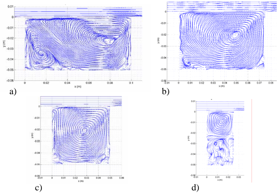
Figure 4: Flow streamlines for a) R = 2 , b) 1.5, c) 1 and d) 0.5, F = 6 and Re between 5 933 and 1 483.
