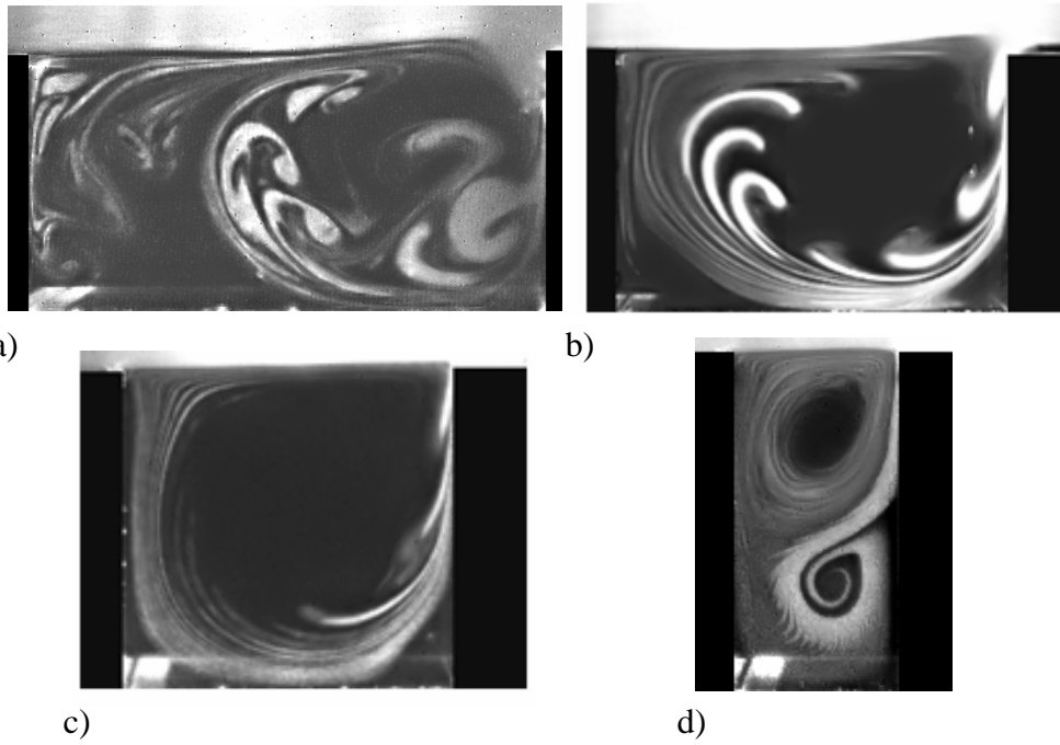
Figure 3: Flow visualizations for a) R = 2 , b) 1.5, c) 1 and d) 0.5, F = 6 and Re between 5 933 and 1 483.
