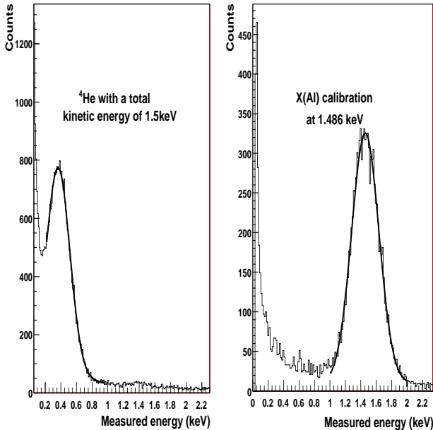
FIG. 2: Spectra of 1.5 keV total kinetic energy ^4\text{He} (left) and 1.486 keV X-ray of ^{27}\text{Al} (right) in ^4\text{He} + 5\% \text{C}_4\text{H}_{10} mixture at 700 mbar. The comparison of the energy measured between these two spectra gives the quenching factor of Helium in ^4\text{He} + 5\% \text{C}_4\text{H}_{10} mixture at 700 mbar.
