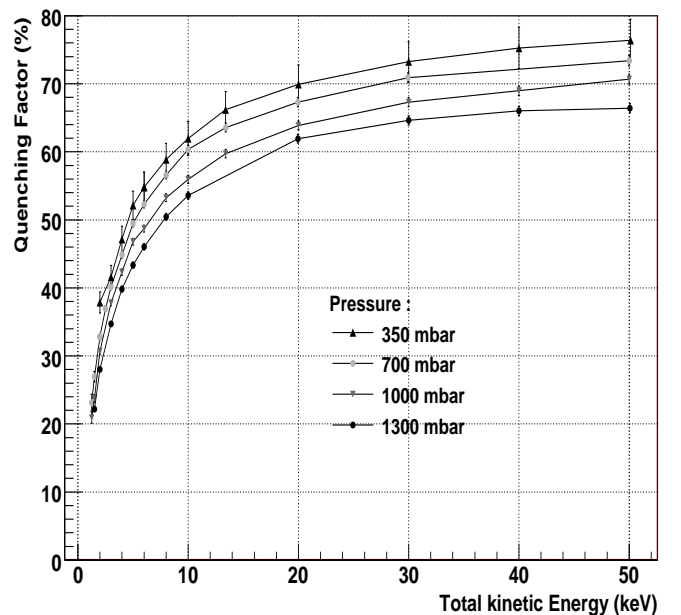
FIG. 3: ^4\text{He} quenching factor as a function of ^4\text{He} total kinetic energy (keV) for 350, 700, 1000 and 1300 mbar, in the case of ^4\text{He} in ^4\text{He} + 5\% \text{C}_4\text{H}_{10} mixture. Measured data are presented with error bars included mainly dominated by systematic errors. Straight line segments between experimental points help to separate the different series of measurements
