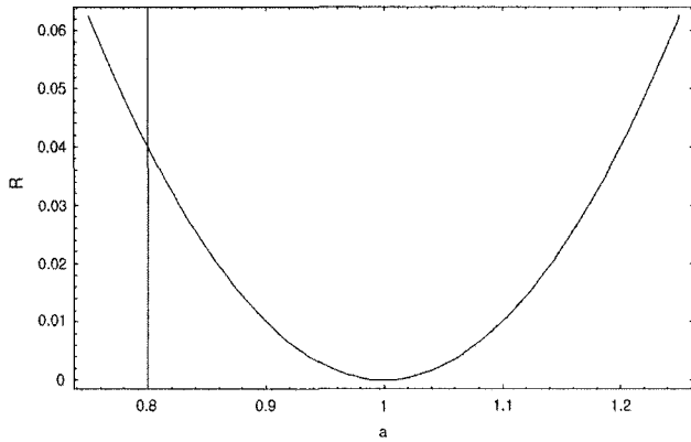
FIG. 6. Evolution of the ratio of the third-harmonic irradiances R = \frac{I_{3\omega, \text{SiO}_2/\text{def}}}{I_{3\omega, \text{air}/\text{SiO}_2}} versus the ratio of the third-order susceptibilities a = \frac{\chi_{\text{def}}^{(3)}}{\chi_{\text{SiO}_2}^{(3)}} .
