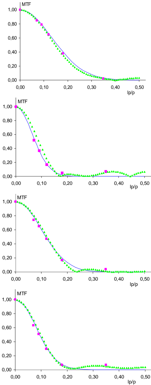
Fig. 10. Comparison of the MTF from the pinhole ( \blacktriangle ), the practical MTF ( \blacksquare ) and the reference MTF ( \text{---} ). Four PSF with different FWHM are used, from top to bottom (FWHM = 3, 4, 5 & 6 pixels).
