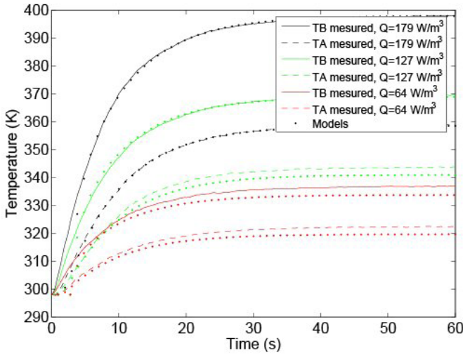
Fig. 11. Comparison between transient part of simulations and experimental measurements for three heat sources ( Q = 179W/m^3 was used for the identification whereas Q = 127W/m^3 and Q = 64W/m^3 were used to check the validity of the results).
