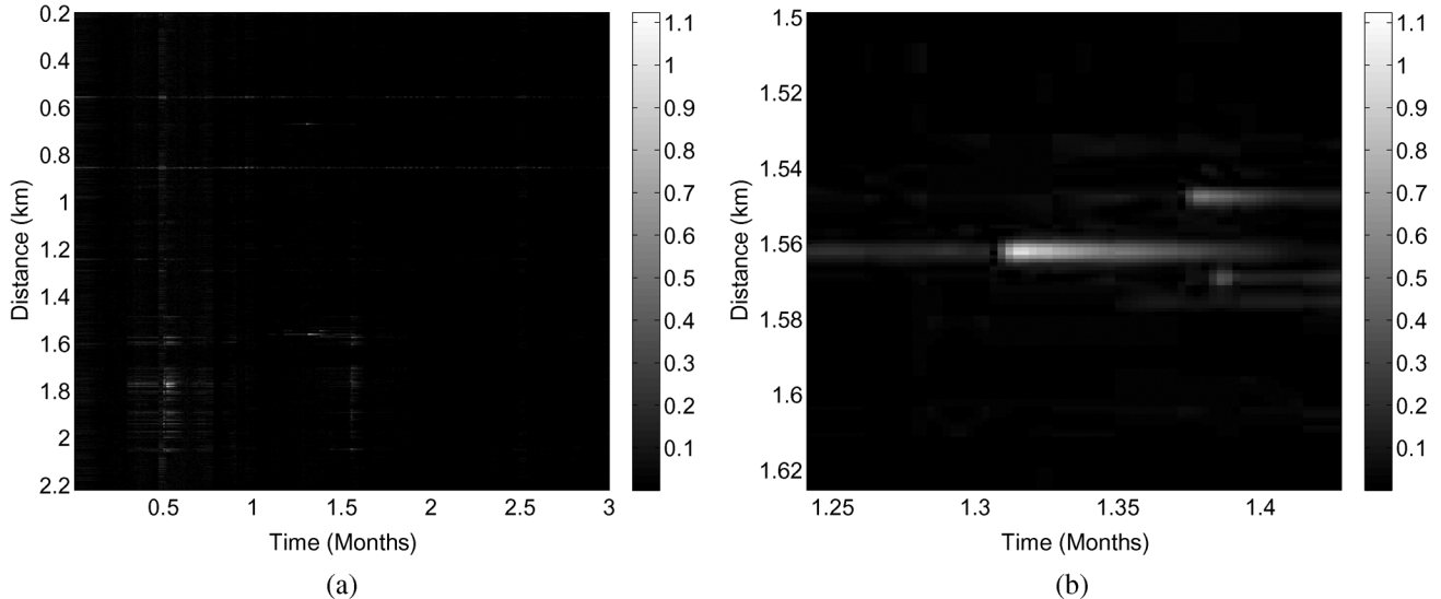
Fig. 9. Residue for the data with spatial gradient taken for a window size of 14 days and an index 142. (a) Envelop of ICA residue. (b) Zoom of (a) in the vicinity of leakages.
