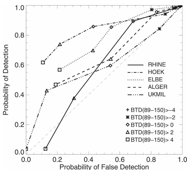
FIG. 12. ROC diagram for BTD between the 90- and 150-GHz channels over land.
