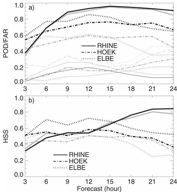
FIG. 10. Time evolution of (a) the POD (thick lines), the FAR (thin lines), and (b) the HSS of the high-cloud category ( 11\text{-}\mu\text{m} BT < 260 K) calculated for the RHINE, HOEK, and ELBE cases. The gray (black) lines represent the calculation grid point by grid point (area by area).
