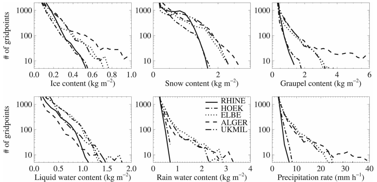
FIG. 3. Distributions of vertically integrated hydrometeor contents ( \text{kg m}^{-2} ) and precipitation rates ( \text{mm h}^{-1} ) for the various cases at the AMSU output times. The bin widths of the ice, snow, graupel, cloud liquid water, and rainwater contents are 0.05, 0.15, 0.3, 0.1, and 0.2 \text{kg m}^{-2} , respectively, and the precipitation rate is 2 \text{mm h}^{-1} .
