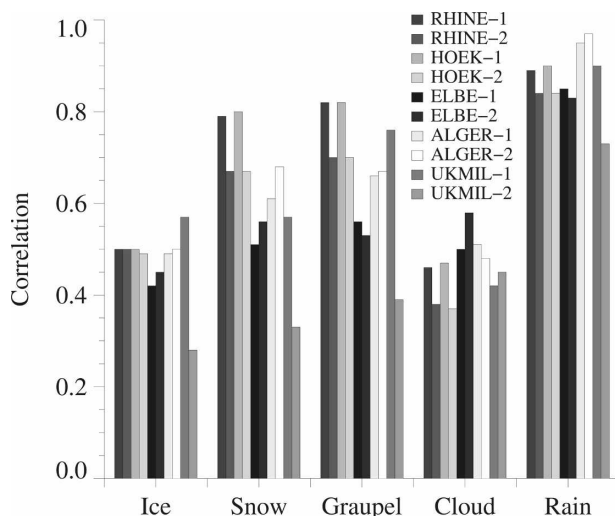
FIG. 5. Correlation of surface precipitation rate with the different integrated hydrometeor contents for the various cases at the two output times.
