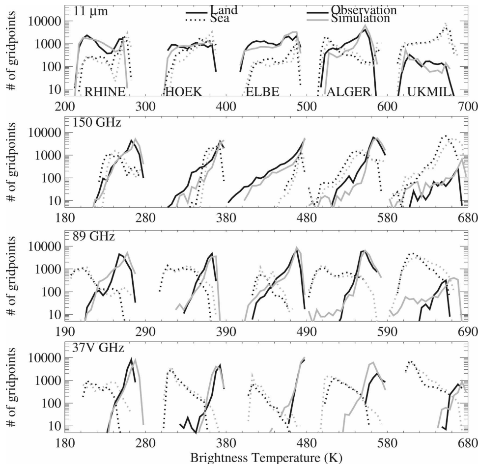
FIG. 8. Observed and simulated BT distributions for the 11- \mu m and 150-, 89- and 37V-GHz channels, separated into land and sea grid points for each case. The bin width is 5 K. The BTs are shifted to the right by 0, 100, 200, 300, 400, and 500 K for the RHINE, HOEK, ELBE, ALGER, and UKMIL cases, respectively.
