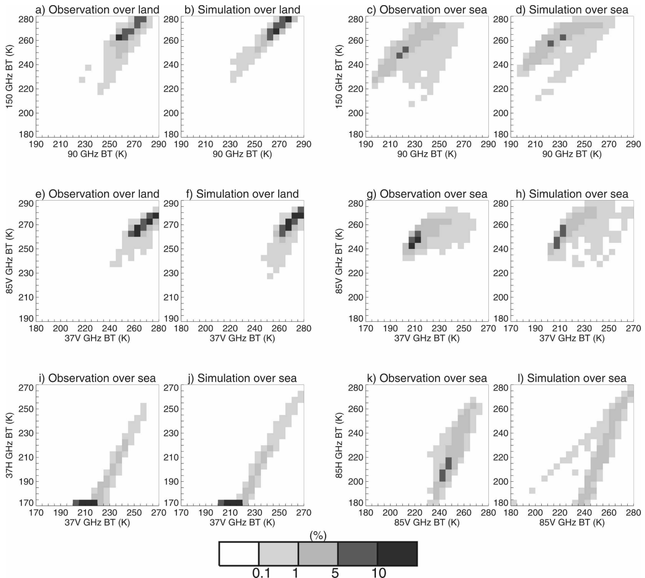
FIG. 9. Observed and simulated joint BT distributions for (top) the 90- and 150-GHz AMSU channels, (middle) the 37V- and 85V-GHz channels, separated into land and sea grid points, and (bottom) the 37V- and 37H-GHz and the 85V- and 85H-GHz channels for grid points over sea only. The bin width is 5 K.
