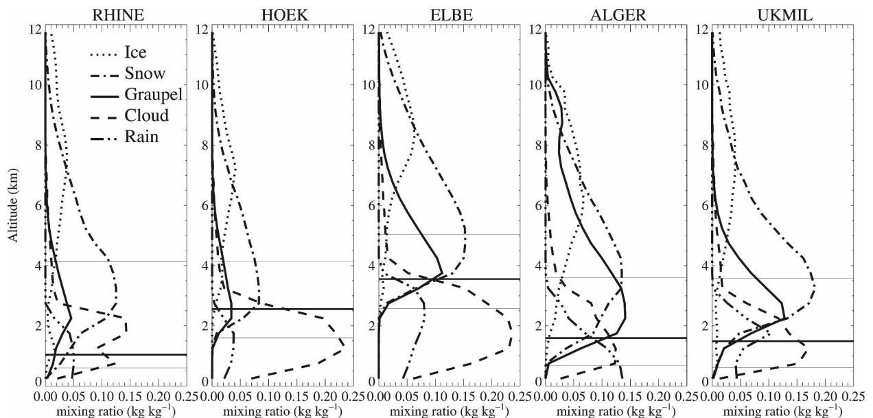
FIG. 4. Mean hydrometeor vertical profiles for the different cases at the AMSU output times. Averages are calculated only from hydrometeor contents that are not null. The horizontal thick (thin) line represents the mean (extreme) altitude(s) of the 0^{\circ}\text{C} isotherm.
