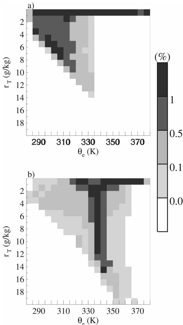
FIG. 6. Conserved-variable ( \theta_e - r_T ) diagrams of the (a) current and (b) GPROF databases obtained from all the tropospheric levels.
