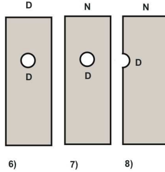
FIGURE 2. The boundary conditions provide the eigenvalue perturbation of order \varepsilon^2 .
