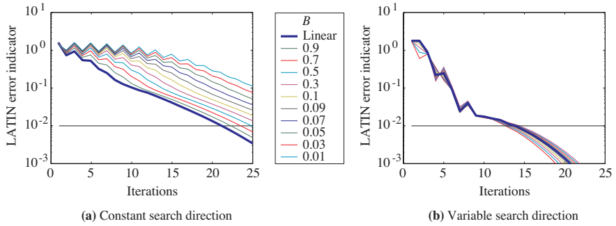
Fig. 2. Variable rigidity
