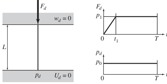
Fig. 1. The force-driven test problem
