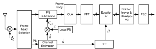
Figure 2. Block diagram of DTMB receiver
