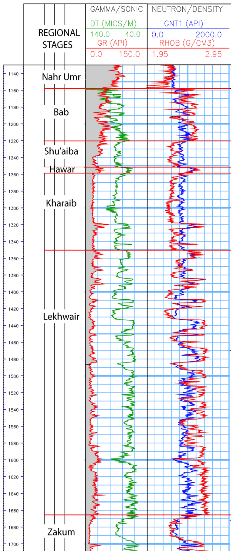
Figure 8: Kahmah section in Lekhwair well N° 7, onshore Oman (modified from HUGHES CLARKE, 1988, and MOHAMMED et alii , 1997).
