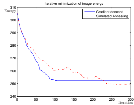
(b) Energy evolution for GD and SA
