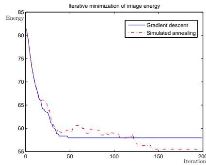
(c) Energy evolution for GD and SA
