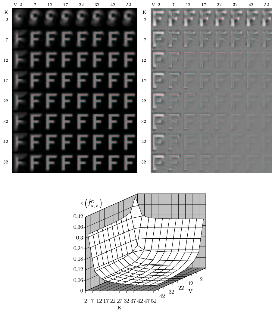
FIG. 6. Evolution of reconstruction of a binary image of the lettre F with the C-Afnt algorithm for varying dimensions K (lines) and V (columns) and corresponding mean square reconstruction error.
