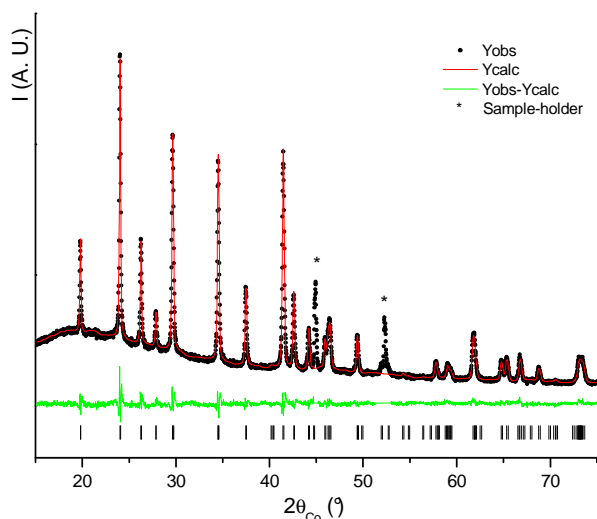
Fig. 4: Comparison of the experimental and calculated X-ray diffraction patterns of \text{Fe}_{800} recovered after 100 cycles of an \text{Li} \parallel \text{C-LiFePO}_4 ( \text{Fe}_{800} ) cell between 2 and 4.5 V vs. \text{Li}^+/\text{Li} , at a C/20 rate and at RT ( \text{Fe}_{800}\text{-RT-100cycles} ).
