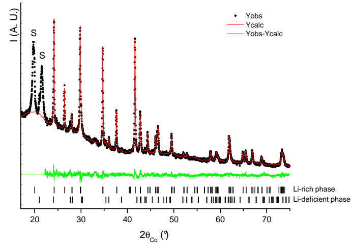
Fig. 5: Comparison of the experimental and calculated X-ray diffraction patterns of \text{Fe}_{800} recovered after 100 cycles of a \text{Li} \parallel \text{C-LiFePO}_4 ( \text{Fe}_{800} ) cell between 2 and 4.5 V vs. \text{Li}^+/\text{Li} , at a C/20 rate and at 40^\circ\text{C} ( \text{Fe}_{800}\text{-}40^\circ\text{C}\text{-}100\text{cycles} ).
