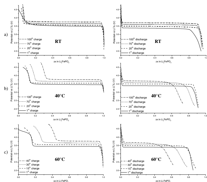
Fig. 1: Cycling curves obtained for Li || C-LiFePO 4 (Fe 800 ) cells in the [2 - 4.5 V] vs. Li + /Li voltage window, at C/20 rate and at RT (a), 40°C (b) and 60°C (c). Comparison of the charge curves and discharge curves obtained during the 1 st , 20 th , 70 th and 100 th cycles for cyclings at RT and 40°C and during the 1 st , 15 th , 30 th and 40 th cycles for cycling at 60°C. Each charge / discharge curve is shifted from the previous reported one of 0.1 V for an easier comparison (note that the first charge and discharge are not shifted).
