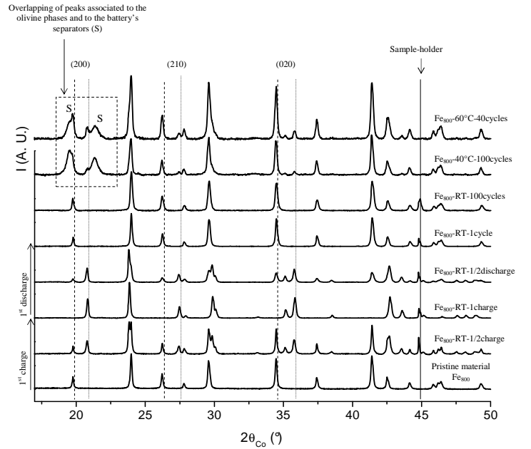
Fig. 3 : Comparison of the X-ray diffraction patterns recorded for the pristine material \text{Fe}_{800} , \text{Fe}_{800} after ½ charge at C/20 and at room temperature ( \text{Fe}_{800}\text{-RT-1/2charge} ), \text{Fe}_{800} after a first charge at C/20 and at room temperature ( \text{Fe}_{800}\text{-RT-1charge} ), \text{Fe}_{800} after a first charge and ½ first discharge at C/20 and at room temperature ( \text{Fe}_{800}\text{-RT-1/2discharge} ), \text{Fe}_{800} at the end of a first electrochemical cycle at C/20 and at room temperature ( \text{Fe}_{800}\text{-RT-1cycle} ), \text{Fe}_{800} after 100 cycles at C/20 rate and at room temperature ( \text{Fe}_{800}\text{-RT-100cycles} ), \text{Fe}_{800} after 100 cycles at C/20 rate and at 40°C ( \text{Fe}_{800}\text{-40°C-100cycles} ) and \text{Fe}_{800} after 40 cycles at C/20 rate and at 60°C ( \text{Fe}_{800}\text{-60°C-40cycles} ).
