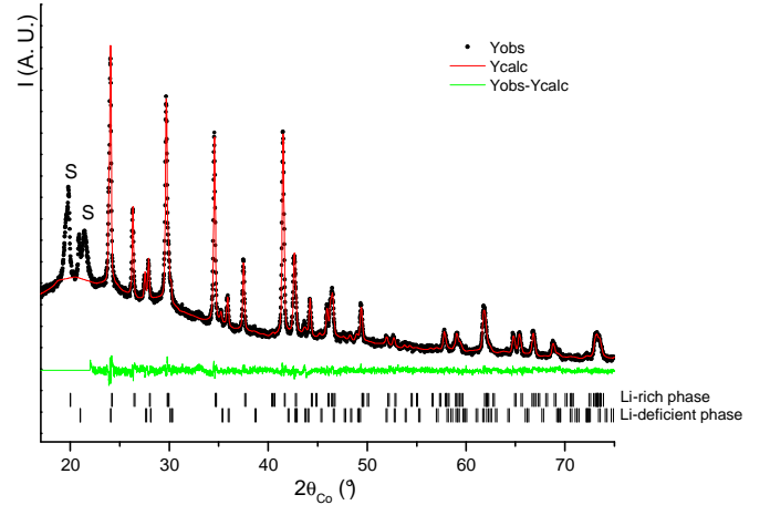
Fig. 6: Comparison of the experimental and calculated X-ray diffraction patterns of \text{Fe}_{800} recovered after 40 cycles of a \text{Li} \parallel \text{C-LiFePO}_4 ( \text{Fe}_{800} ) cell between 2 and 4.5 V vs. \text{Li}^+/\text{Li} , at a C/20 rate and at 60^\circ\text{C} ( \text{Fe}_{800}\text{-}60^\circ\text{C}\text{-}40\text{cycles} ).
