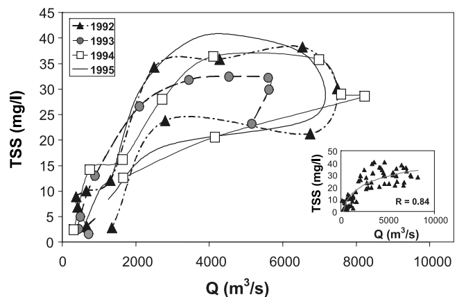
Figure 4. The Oubangui River at Bangui station: relationship between monthly TSS concentrations and water discharges from 1992 to 1995 showing clockwise hysteresis.
