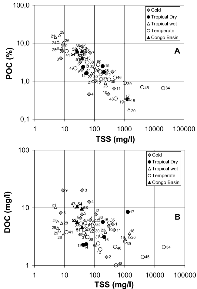
Figure 2. Distribution of mean annual (a) POC contents and (b) DOC concentrations in the world's rivers clustered by climate (data from Meybeck [1993] and Meybeck and Ragu [1996] unless specified below by superscripts denoting the following: a, Weibezahn et al. [1990]; b, Gordeev et al. [1996]; c, Carson et al. [1998]; d, Holmes et al. [2002]; e, Lobbess et al. [2000]; f, Köhler et al. [2003]; g, Seyler et al. [2005]; and h, this study). Cold: Mackenzie (1 b,c ), Alpine Rhone (2), N Dvina (3), Pechora (4), Ob (5 d,f ), Lena (6 b,d ), Amur (7), Yenisey (8 d,e,f ), Moose (9), Yukon (10), Beni (11), Mamore (12). Tropical dry: Gambia (13), Orange (14), Zambesi (15), Niger (16), Murray (17). Tropical wet: Nile (18), Ganges (19), Brahmaputra (20), Negro (21 g ), Solimoes (22 g ), Madeira (23 g ), Trombetas (24 g ), Tapajos (25 g ), Xingu (26 g ), Amazone (27 g ), Caroni (28), Caura (29), Orinoco (30 a ), Sanaga (31), Tuy (32), Parana (33). Temperate: Huang He (34), Danube (35), Loire (36), Mississippi (37), Ohio (38), Peace (39), Rhine (40), St. Lawrence (41), Kuban (42), Don (43), Dniepr (44), Choroch (45), Changjiang (46), Pee Dee (47), Rioni (48), Seine (49), Rhone (50). Congo Basin: Mpoko (51 h ), Oubangui (52 h ), Ngoko (53 h ), Congo outlet (54 h ).
