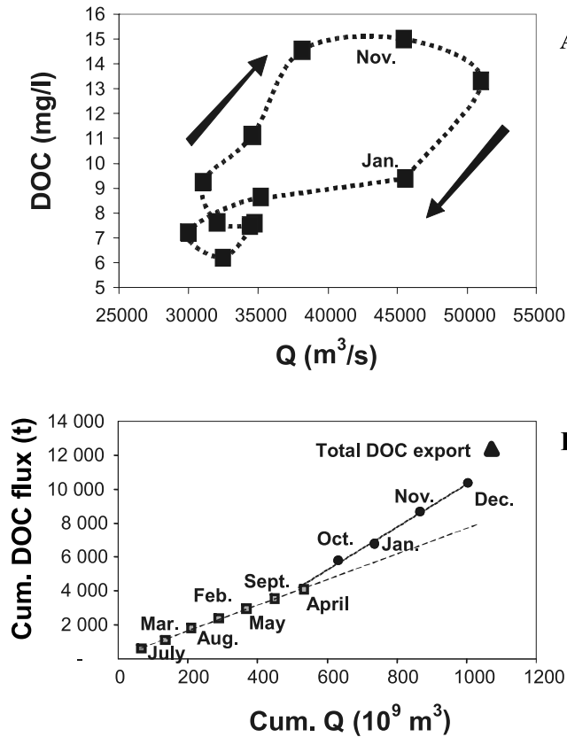
Figure 8. The Congo River at Kinshasa/Brazzaville station: (a) relationship between monthly “average” DOC concentrations versus mean monthly water discharges; (b) temporal variability of DOC fluxes as a function of “cumulative monthly DOC fluxes versus cumulative monthly water discharges.”
