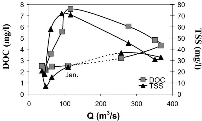
Figure 6. Mpoko River at Nzongo station: relationship between monthly “average” TSS and DOC concentrations versus mean monthly water discharges.
