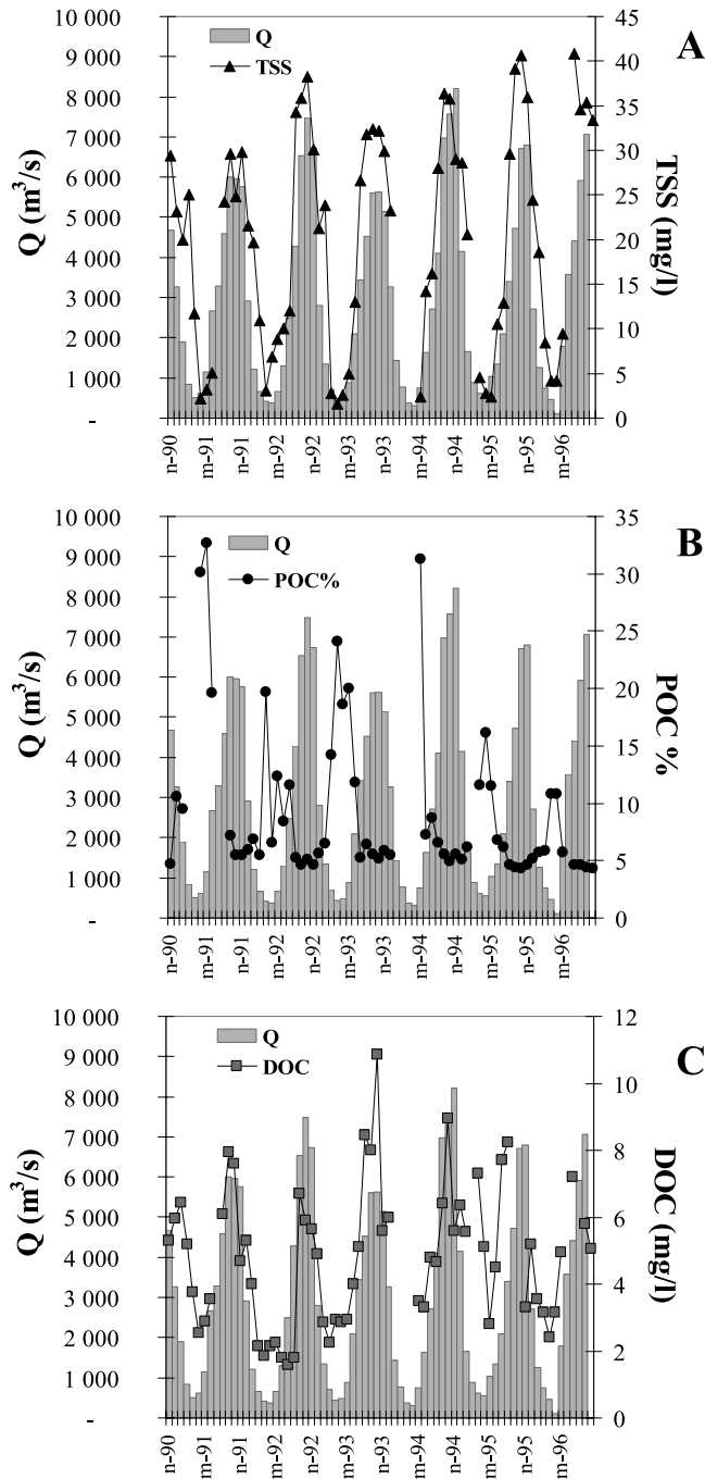
Figure 3. The Oubangui River at Bangui station: time series of monthly water discharges (Q) and (a) TSS concentrations, (b) POC contents in TSS, and (c) DOC concentrations for six hydrological cycles (from November 1990 to October 1996).
