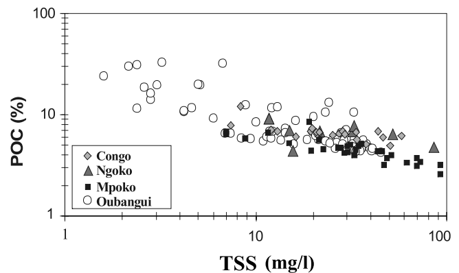
Figure 9. Variation of individual POC contents versus TSS concentrations for the four stations of the Congo-Zaire Basin.
