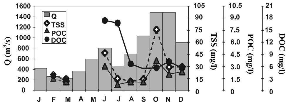
Figure 7. Ngoko River at Moloundou station: temporal distribution of monthly water discharges, TSS, POC, and DOC concentrations.
