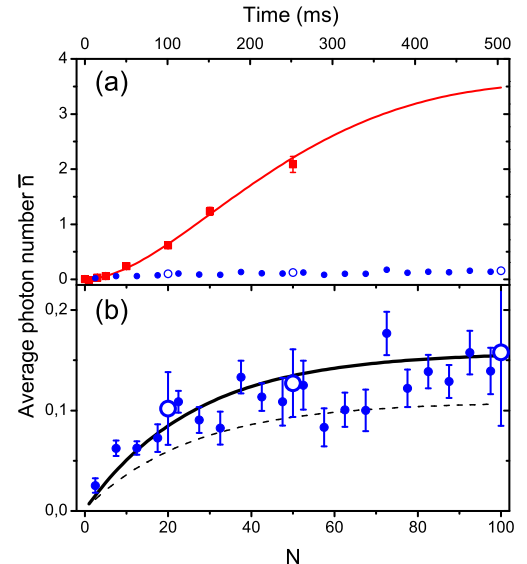
FIG. 3: (a) Average photon number \bar{n} in C as a function of the number N of injection pulses (bottom axis). The top axis gives a time scale for the complete sequence, including injection and measurement times. The red squares correspond to the uninhibited field growth, without measurements between injections (statistical error bars for N < 50 are smaller than point size). The initial evolution is quadratic. The line is a fit providing a precise calibration of the injection pulse amplitude. The blue dots result from atomic spin tomography performed between injection pulses. The field growth is inhibited by the quantum Zeno effect. The open circles correspond to QND measurements of the photon number using 200 atomic detections at the end of sequences with 20, 50 and 100 injection/measurement cycles. (b) Inhibited field evolution with an expanded vertical scale (blue dots in a). The error bars reflect the statistical noise. The solid and dotted black lines are theoretical predictions (see text). The initial growth is now linear.
