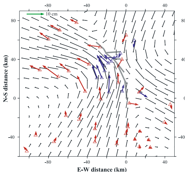
Figure 6. Postseismic horizontal displacements from 1992 to 1999 relative to stable North America. Measurements from the USGS (blue symbols) [ Savage and Svarc, 1997 ] were used in the inversion and the SCEC data (SOPAC: http://sopac.ucsd.edu/dataArchive/ ) (red symbols) were not. Black arrows show the velocities predicted by our model. Thick lines show the simplified fault geometry [ Fialko, 2004b ] used in this study.
