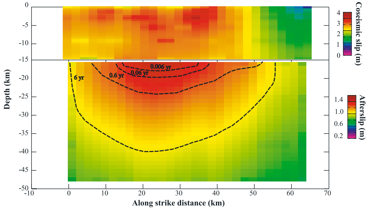
Figure 3. (top) Coseismic slip and (bottom) modeled postseismic slip after 6 years of relaxation. The time evolution of afterslip is represented by isochrons. Each isochron encompasses the zone within which the cumulative slip exceeds 70% of the peak slip at the considered time.
