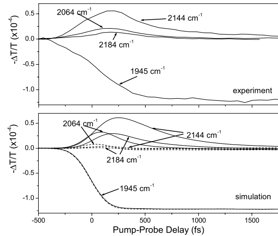
FIG. 2. Differential transmission in MbCO for the four different probes of Fig. 1. Upper panel: Experiment. Pump energies of 180–280 nJ were used. The DT signals were linearly scaled to the average pump energy of 220 nJ. The relative amplitudes are correct within approximately 20%. Lower panel: Calculated signals using a phenomenological model that assume a progressive (quasi-instantaneous) absorption strength change for the CO vibration are shown as solid (dashed) lines.
