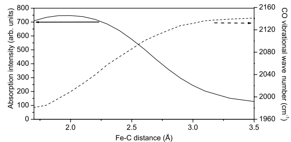
FIG. 3. Density-functional calculations of the CO vibrational absorption intensity (solid line) and frequency (dashed line) using a model system consisting of an iron porphine with a bound CO, an axial and a distal imidazole (see text).
